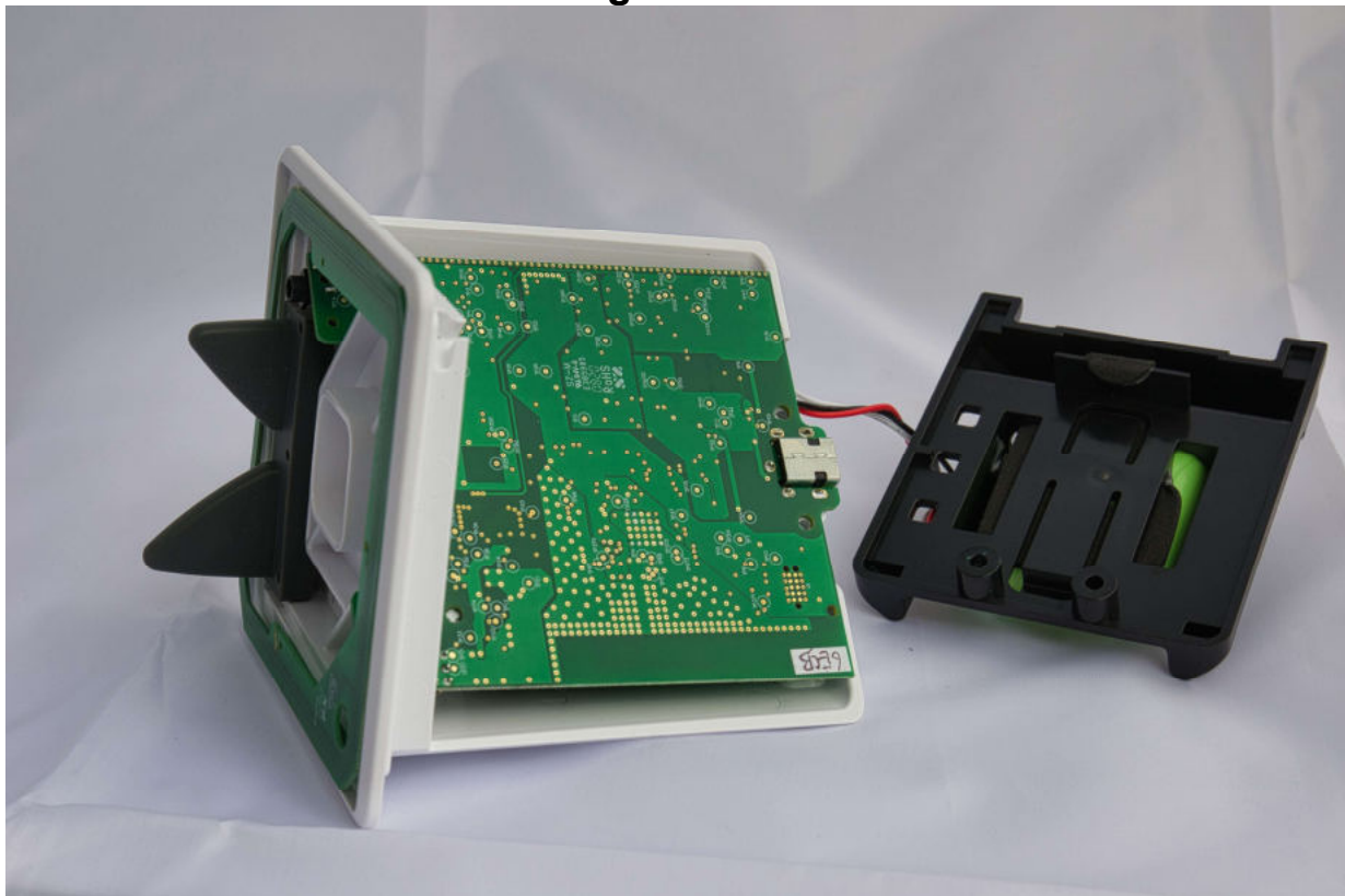
RFID Antenna PCB mounted together with Main PCB in Chassis
