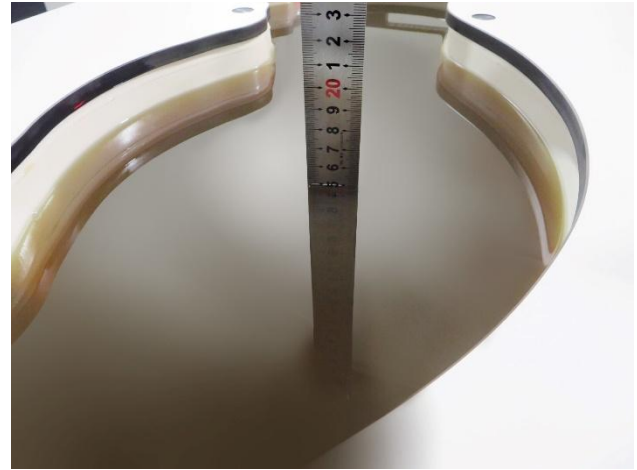
15 cm Depth Head Tissue for ELI Phantom
