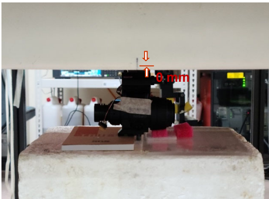
Photograph 5. Body, Position 3, 0mm
