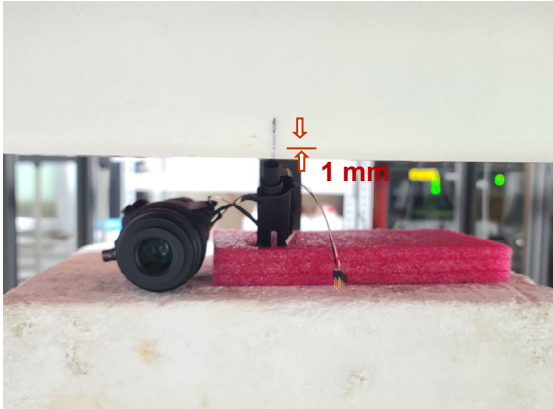
Photograph 1. Body, Position 1, 1mm
