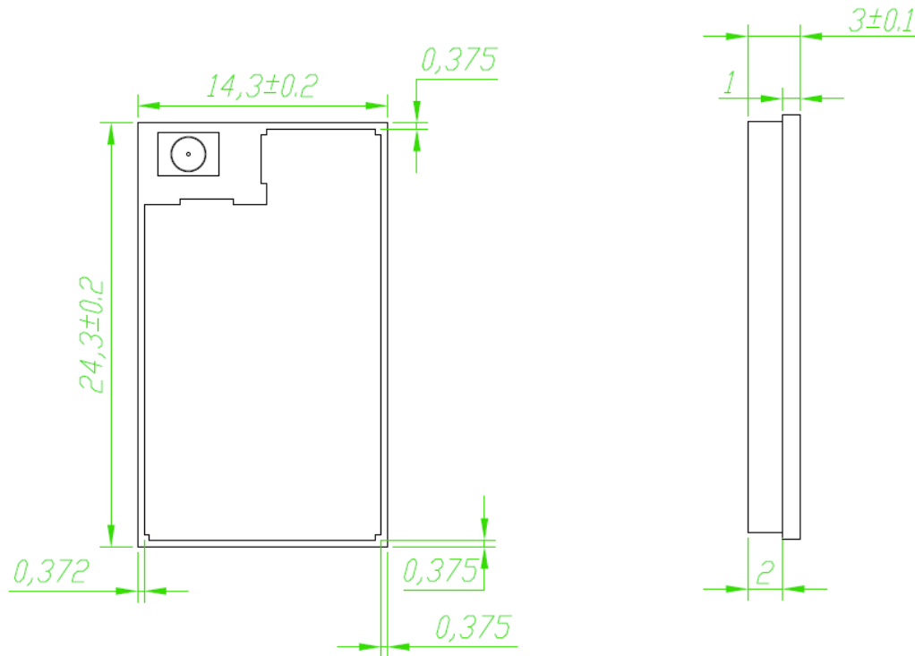
Figure 8: Module Top
