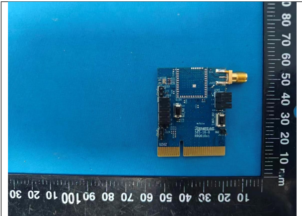
Daughterboard(
