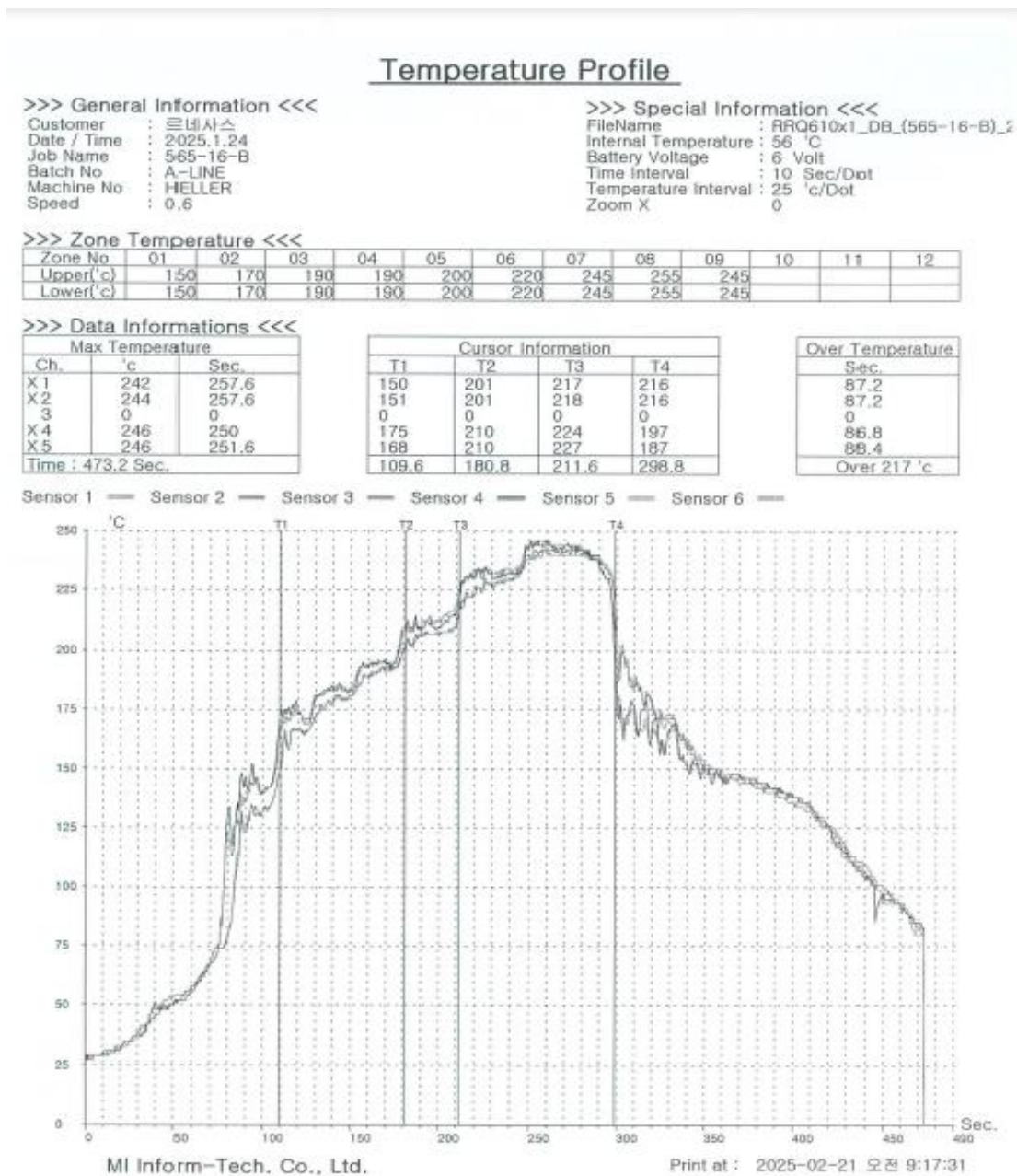
Figure 29. Reflow profile for lead free solder, applied on RRQ61001 daughterboard
