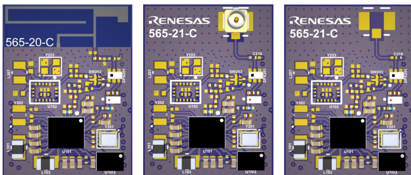
Figure 4. Renesas RRQ61001 modules: RRQ61001-008 (left), RRQ61001-009 (center), and RRQ61001-010 (right)
