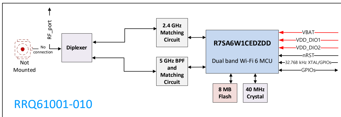
Figure 3. Interconnection of all the physical blocks in RRQ61001-010 module
