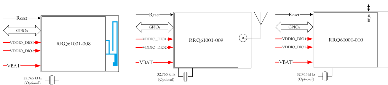
Figure 7. Hardware setup of RRQ61001-008 (left), RRQ61001-009 (center), and RRQ61001-010 (right)
