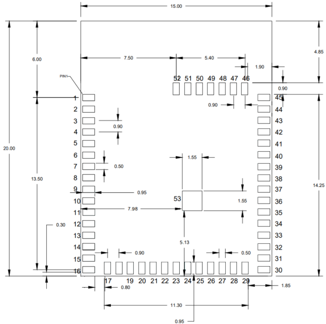
Figure 27. Recommended land pattern (PCB top view, NSMD design)
