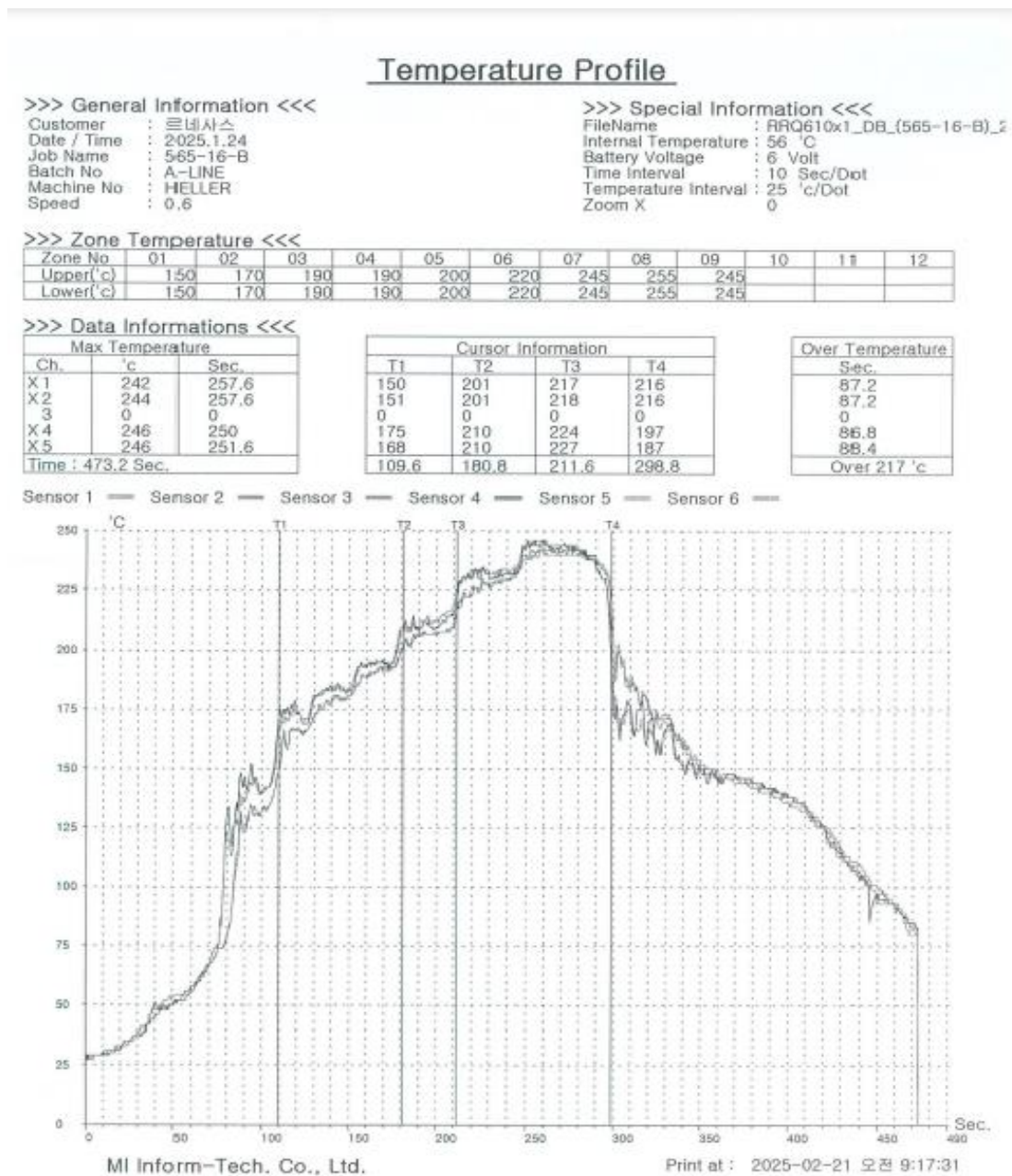
Figure 31. Reflow profile for lead free solder, applied on RRQ61051 daughterboard
