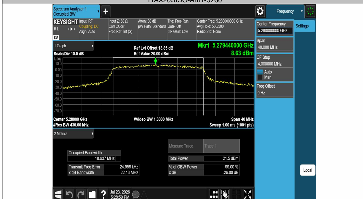
11AX20SISO-Ant1-5280
