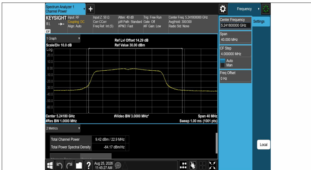
11A-Ant1-5240-PASS
