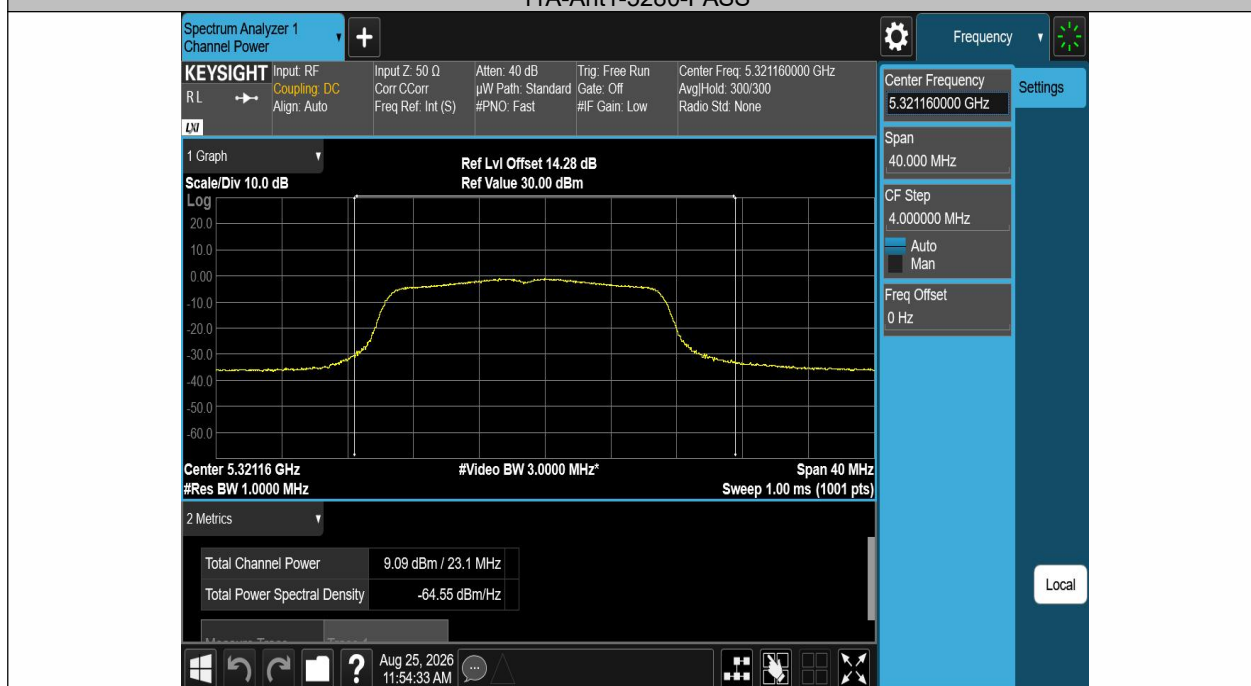
11A-Ant1-5320-PASS
