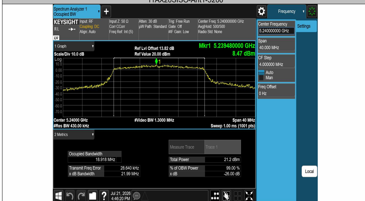
11AX20SISO-Ant1-5240
