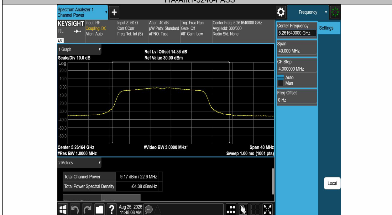
11A-Ant1-5260-PASS
