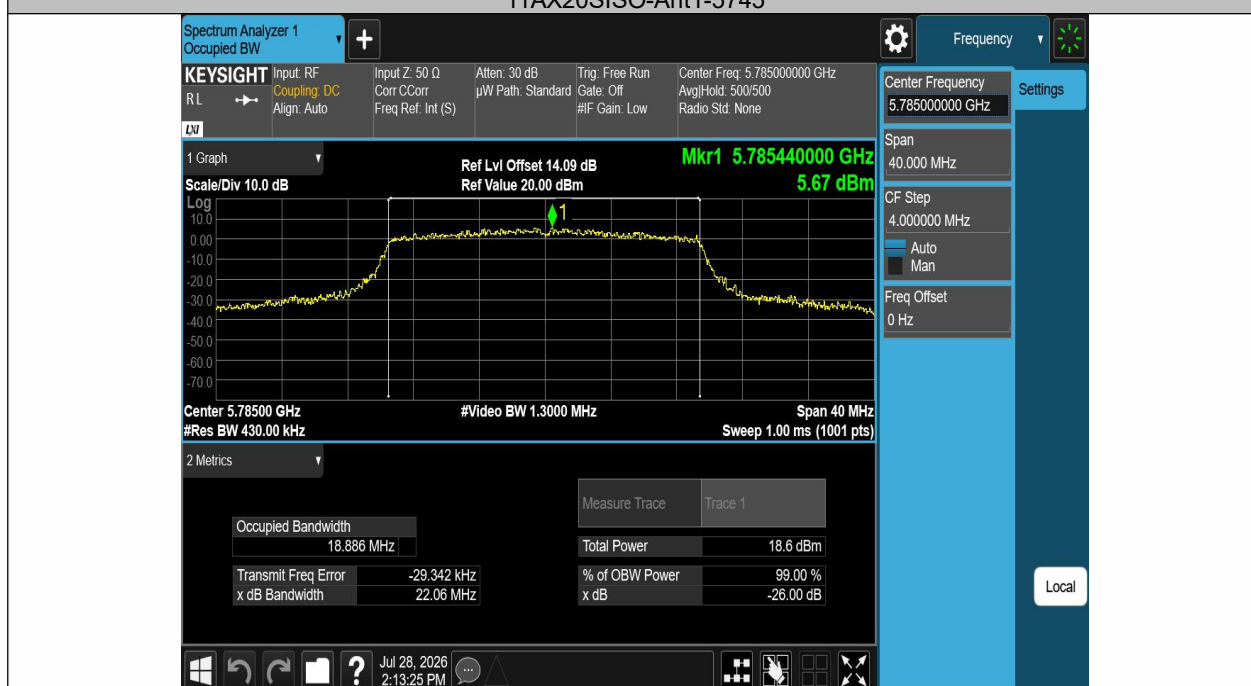
11AX20SISO-Ant1-5785
