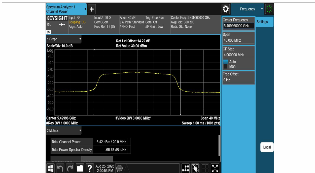
11N20SISO-Ant1-5500-PASS
