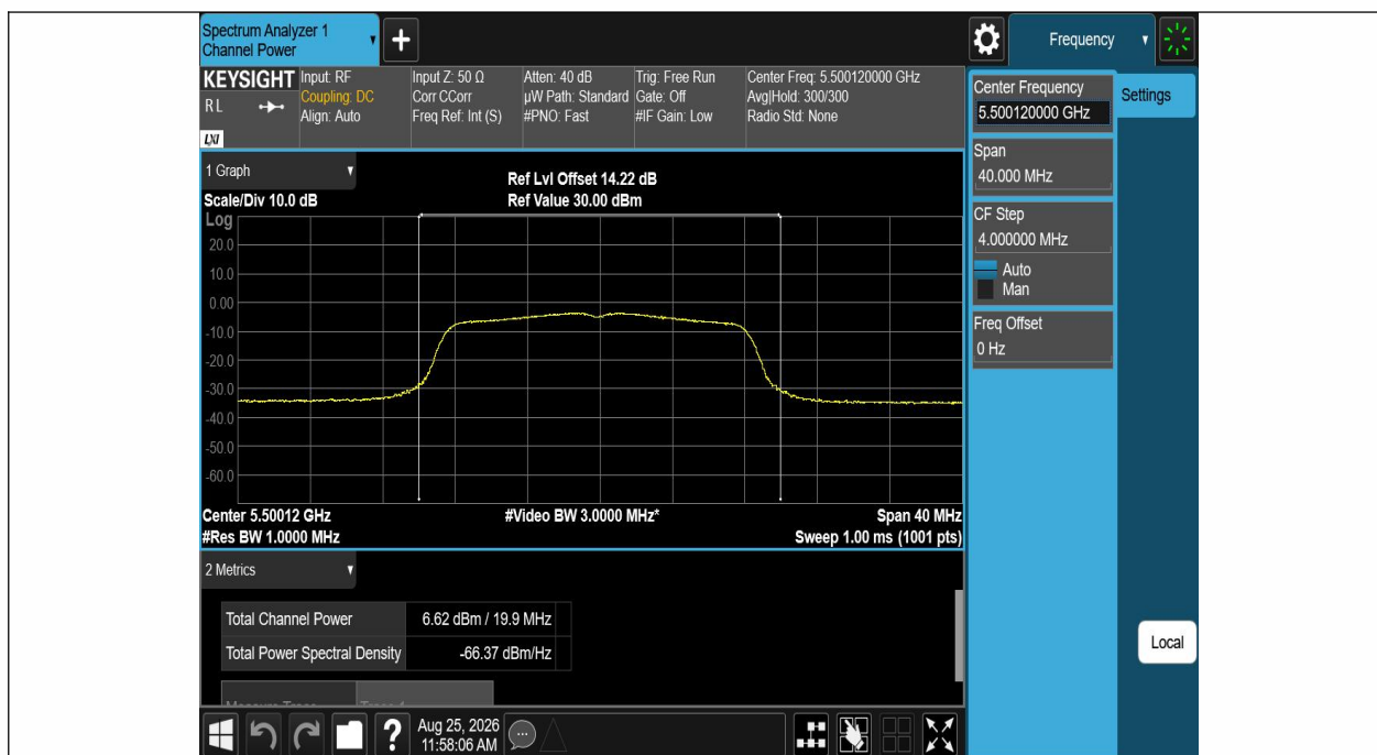
11A-Ant1-5500-PASS
