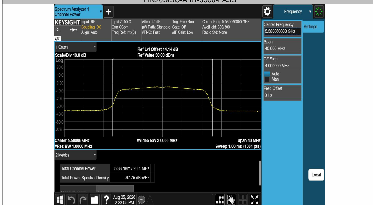
11N20SISO-Ant1-5580-PASS
