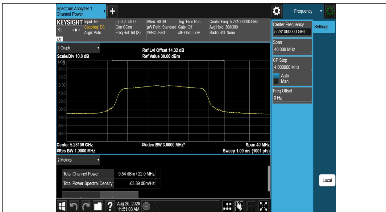
11A-Ant1-5280-PASS
