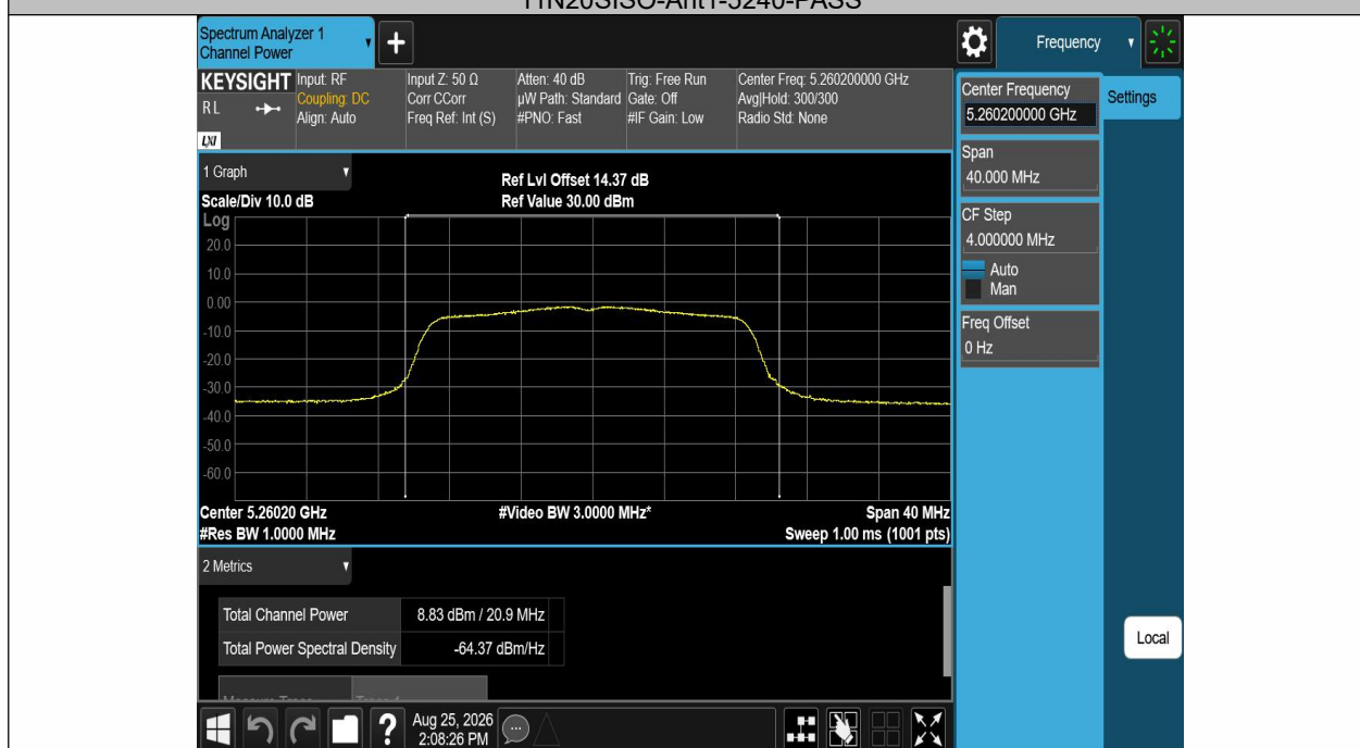
11N20SISO-Ant1-5260-PASS
