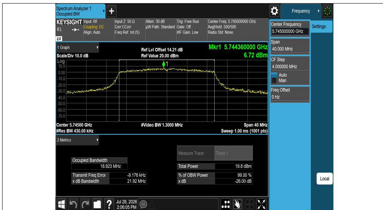
11AX20SISO-Ant1-5745
