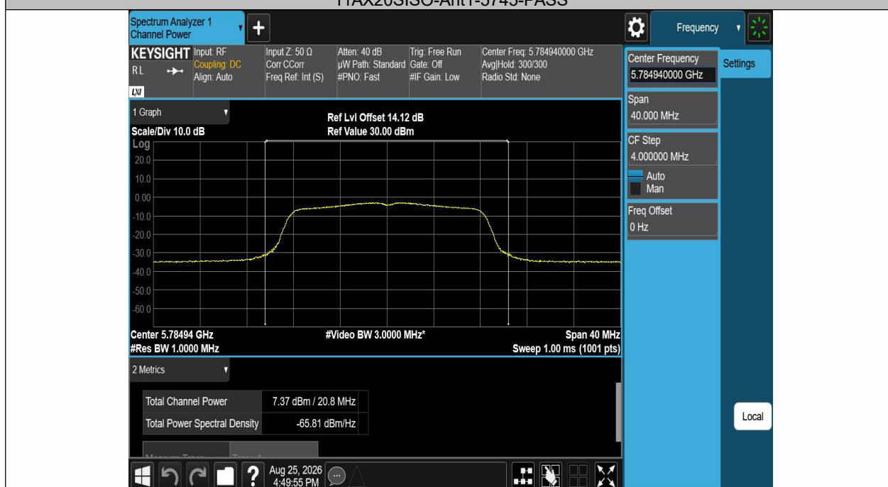
11AX20SISO-Ant1-5785-PASS
