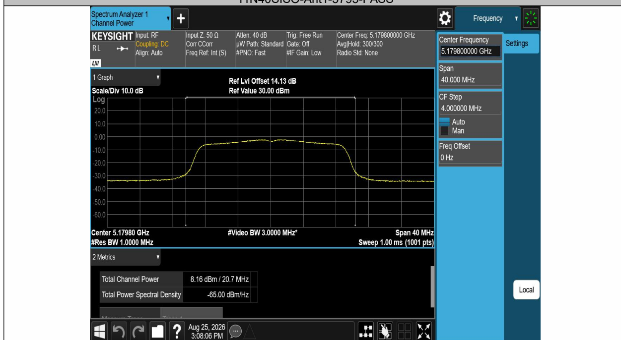
11AC20SISO-Ant1-5180-PASS
