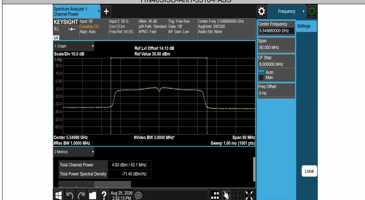
11N40SISO-Ant1-5550-PASS
