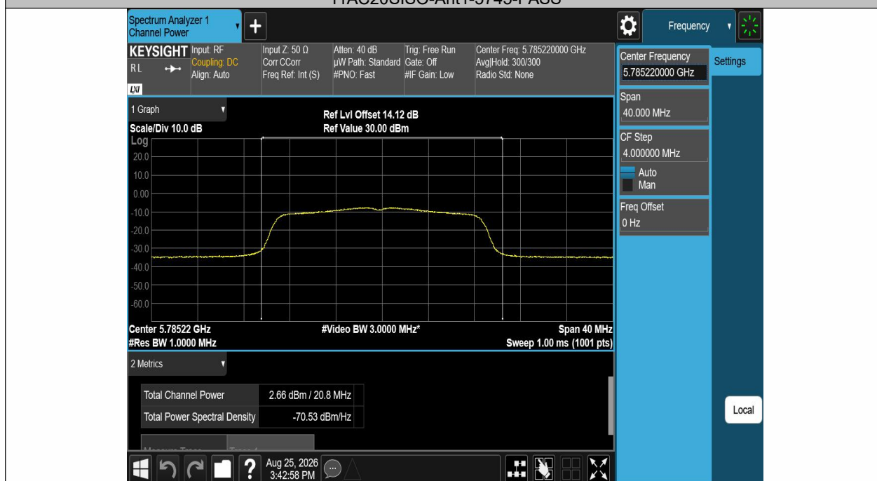
11AC20SISO-Ant1-5785-PASS
