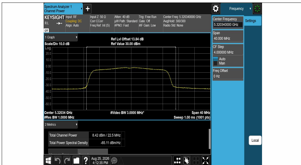
11AX20SISO-Ant1-5320-PASS
