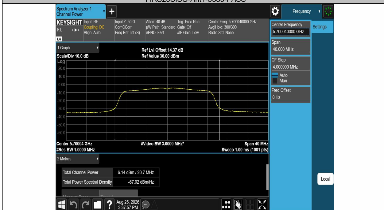
11AC20SISO-Ant1-5700-PASS
