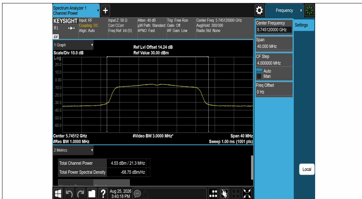
11AC20SISO-Ant1-5745-PASS
