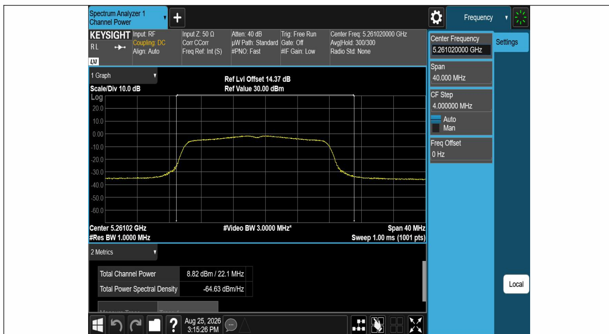
11AC20SISO-Ant1-5260-PASS
