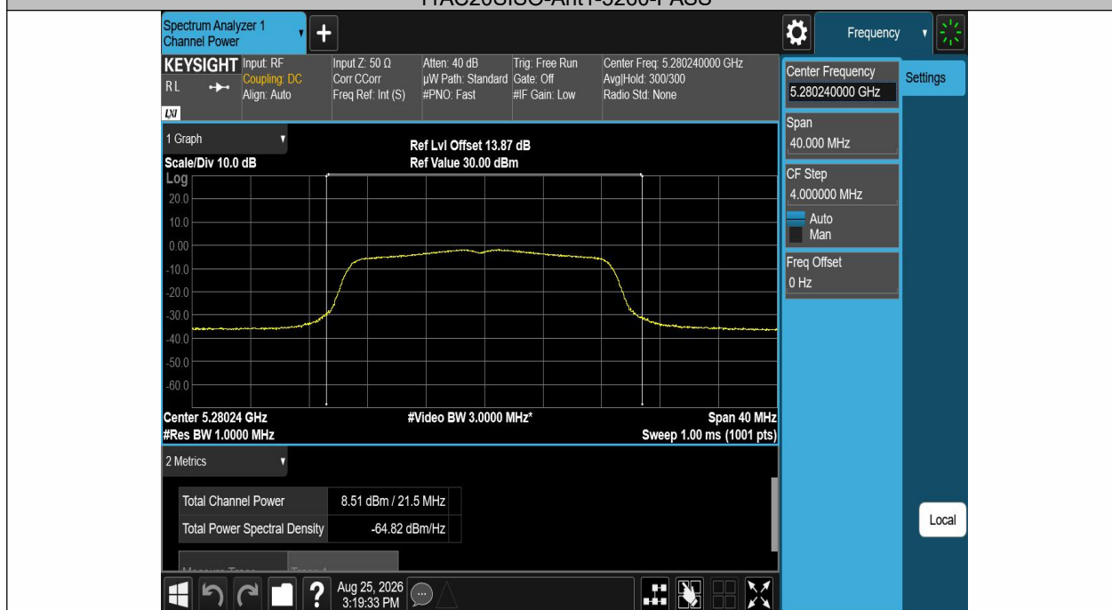
11AC20SISO-Ant1-5280-PASS
