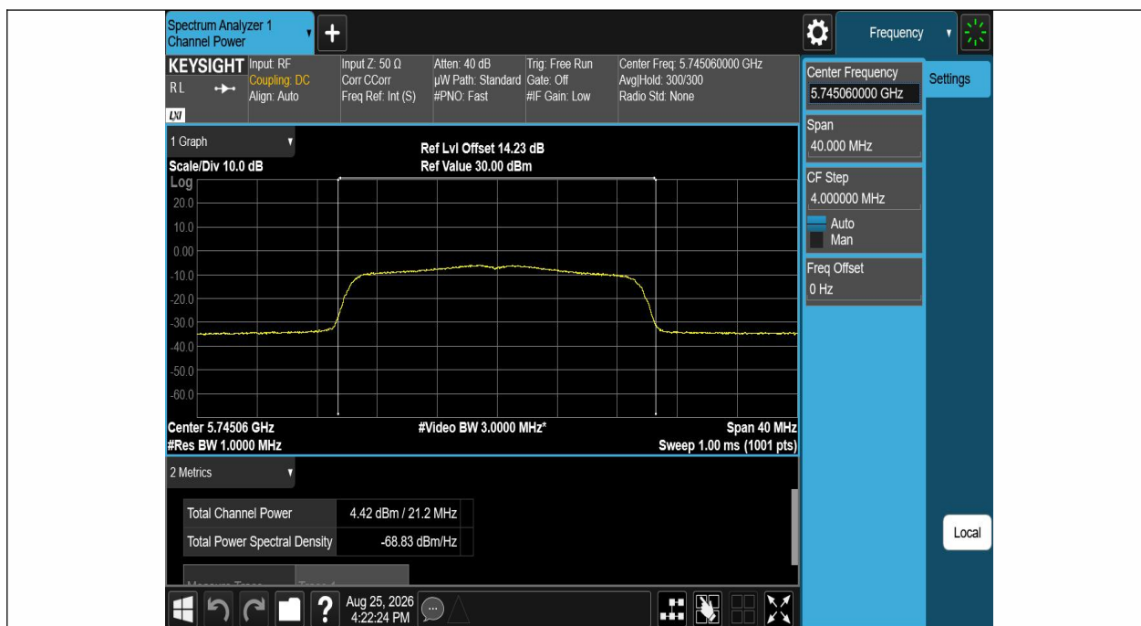
11AX20SISO-Ant1-5745-PASS
