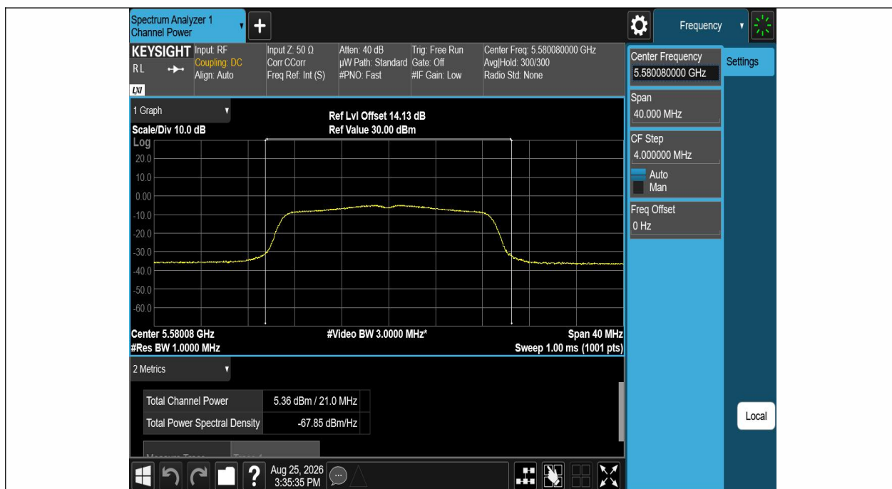
11AC20SISO-Ant1-5580-PASS
