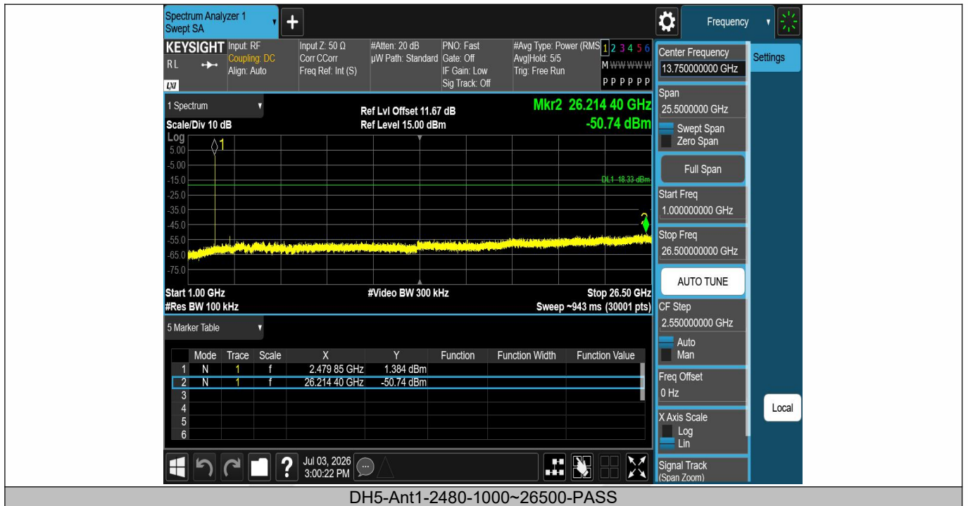
DH5-Ant1-2480-1000~26500-PASS
