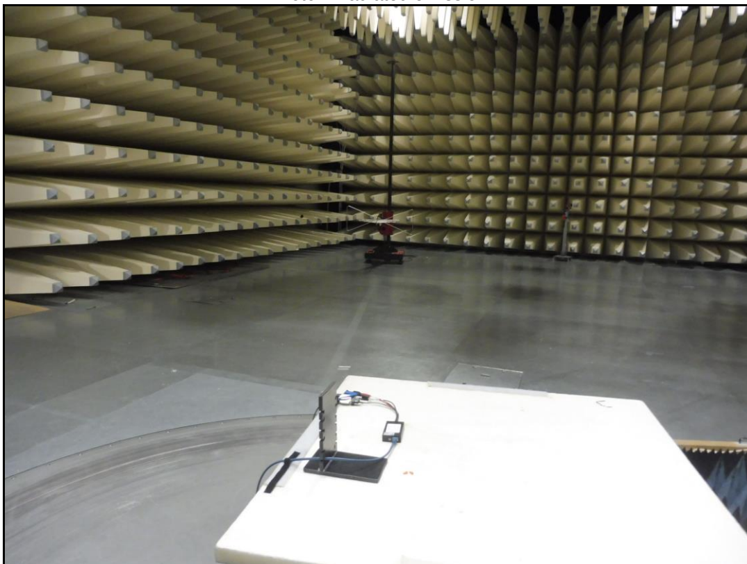
Photo 1: radiated emission
