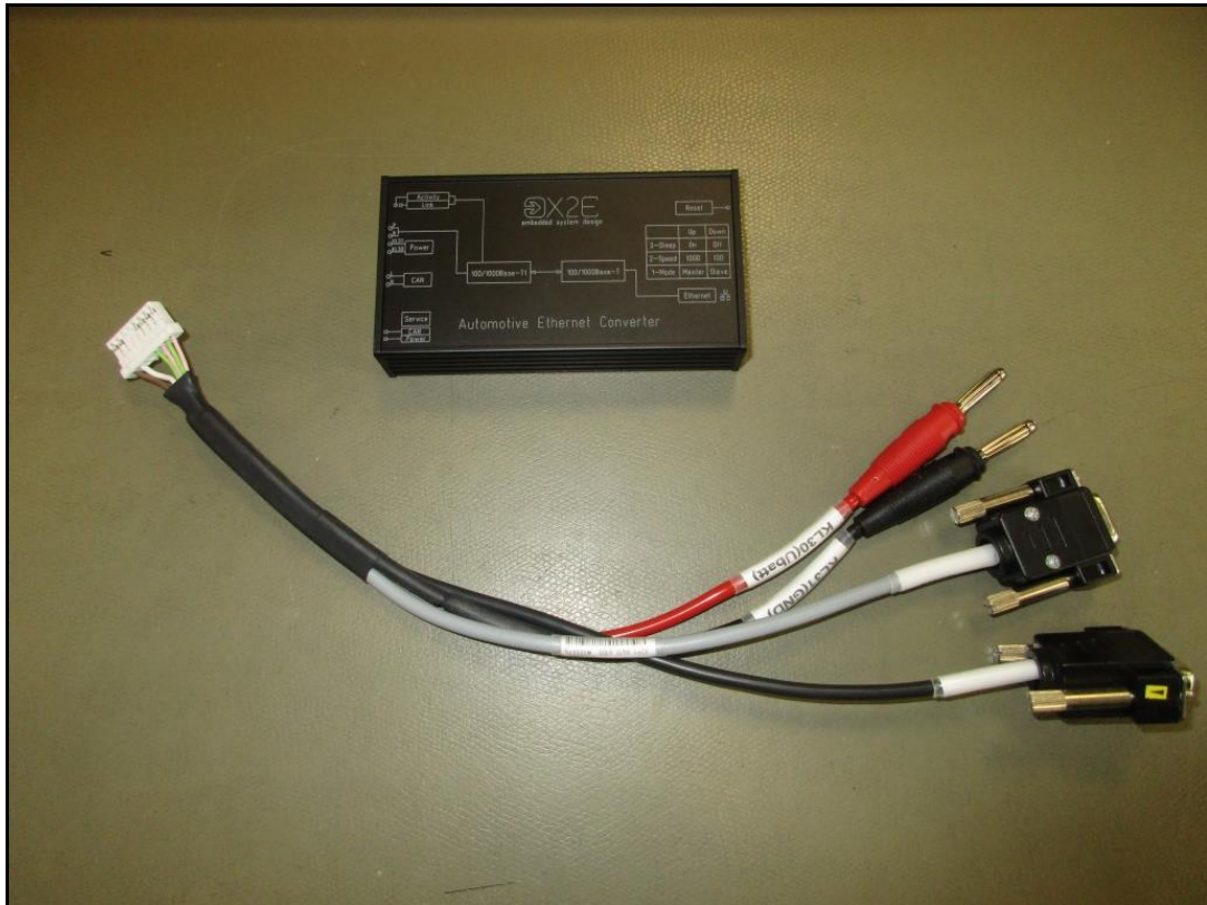
Photo 8: EUT
