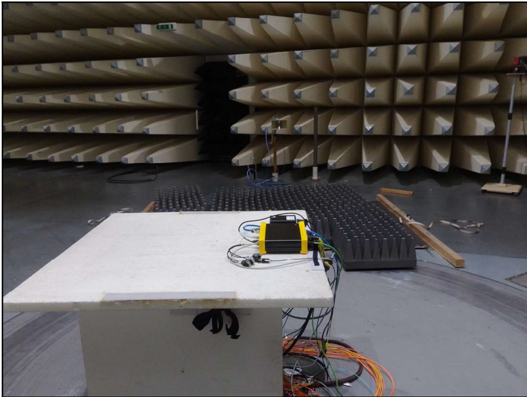
Photo 3: radiated emission
