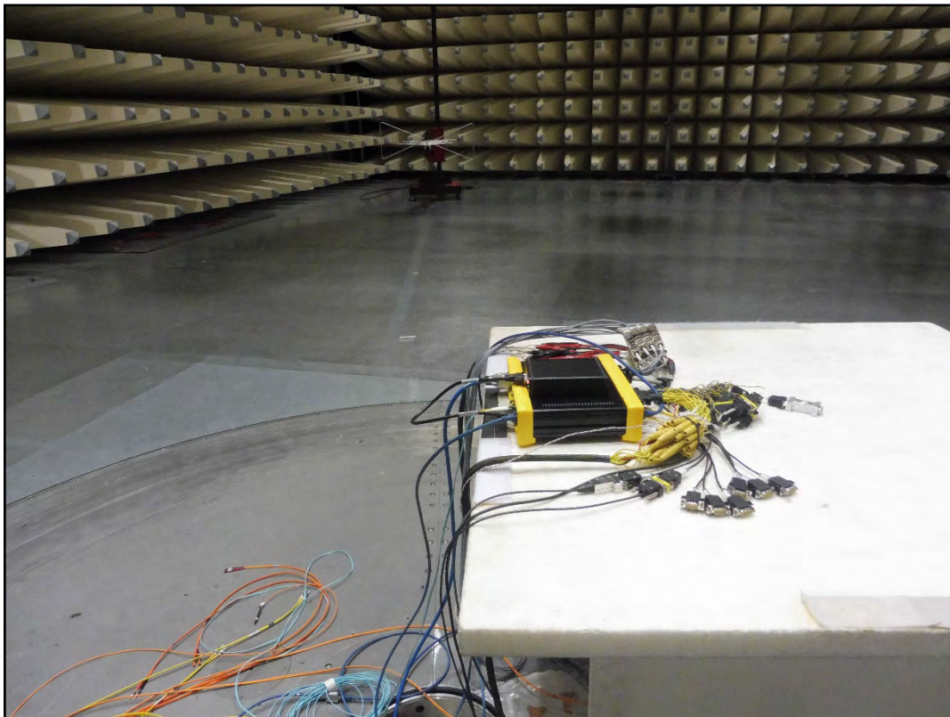
Photo 5: radiated emission
