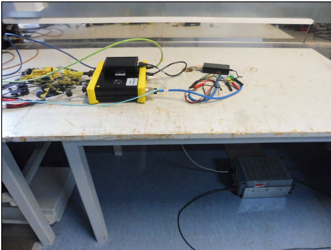
Photo 9: conducted emission
