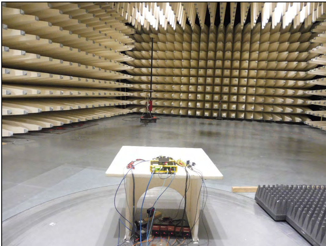
Photo 1: radiated emission
