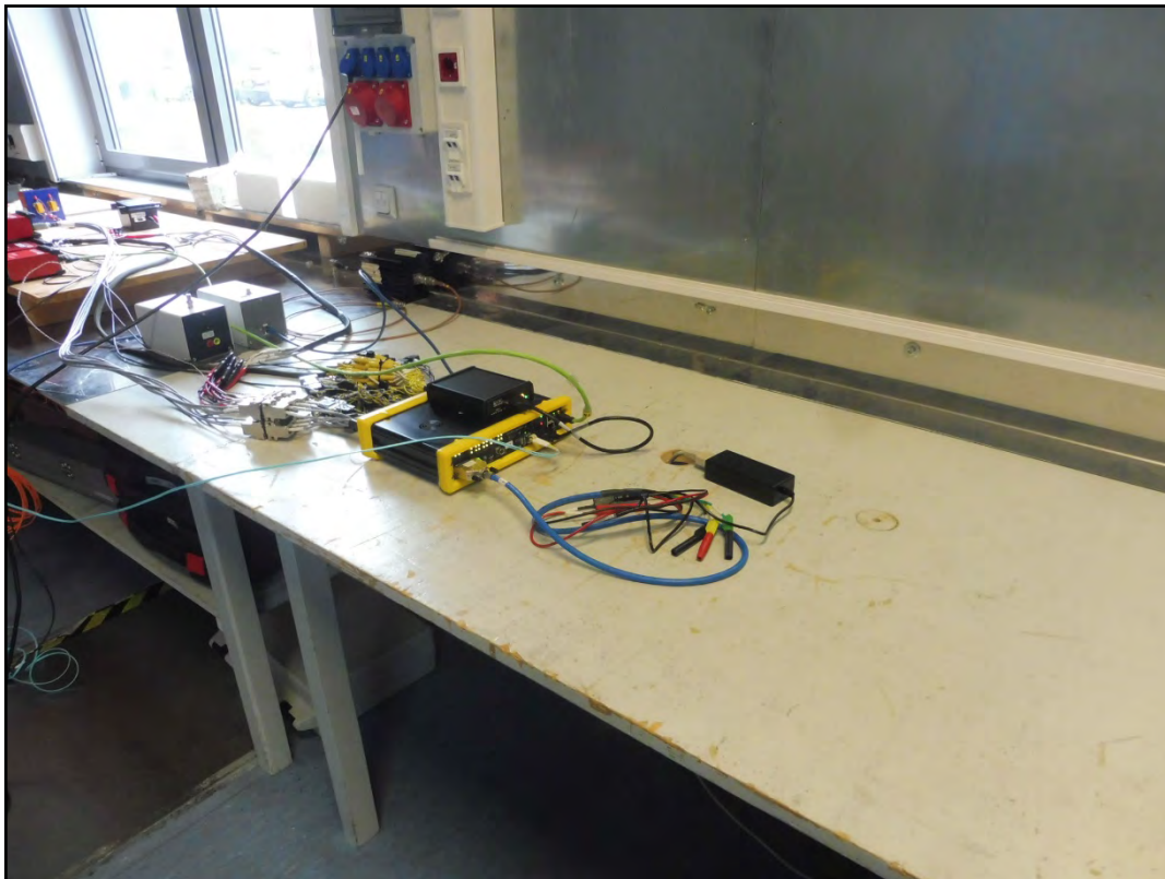
Photo 8: conducted emission
