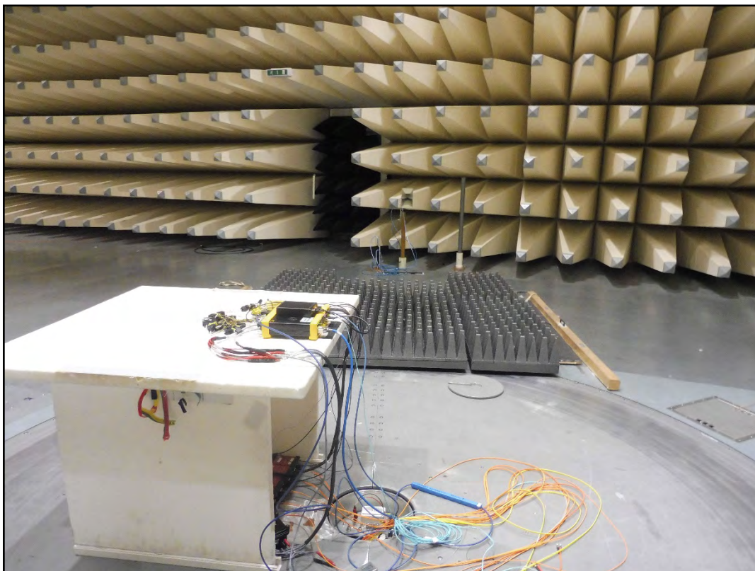
Photo 3: radiated emission
