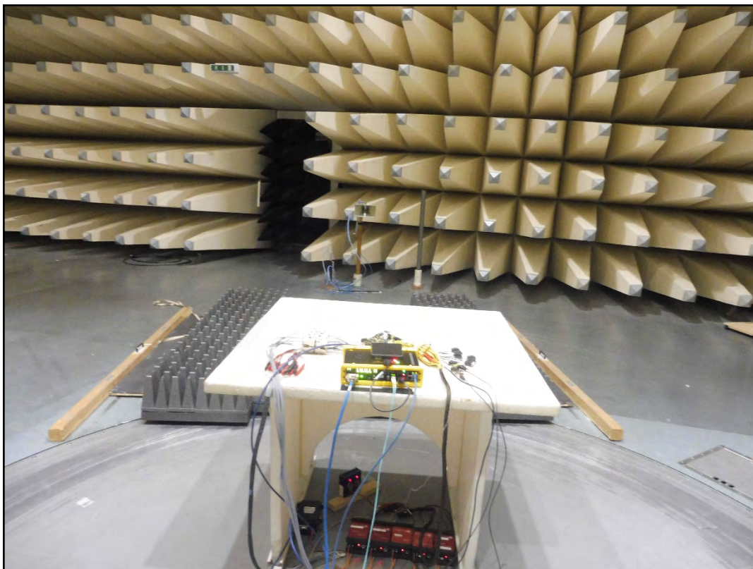
Photo 4: radiated emission
