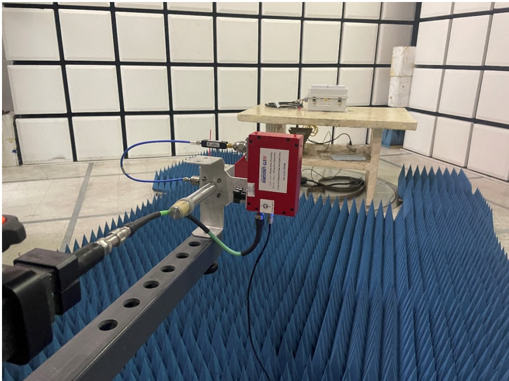
Photo 3: Emissions in frequency range 3-18 GHz
