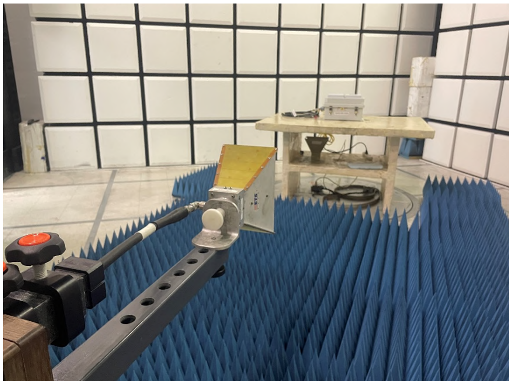
Photo 2: Emissions in frequency range 1-3 GHz
