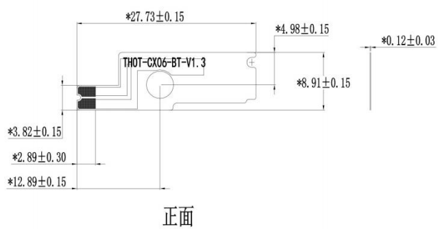
BLE/ANT+ Antenna
