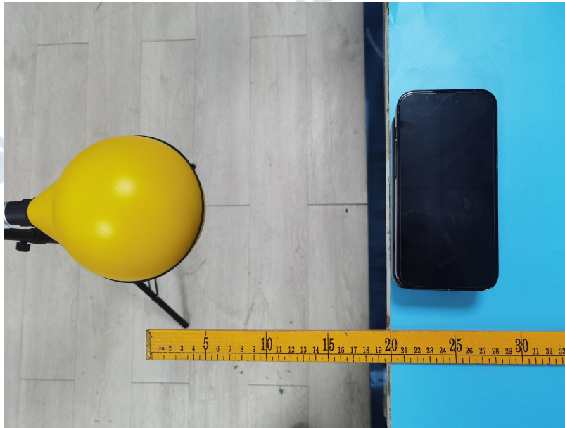
20cm-Left
