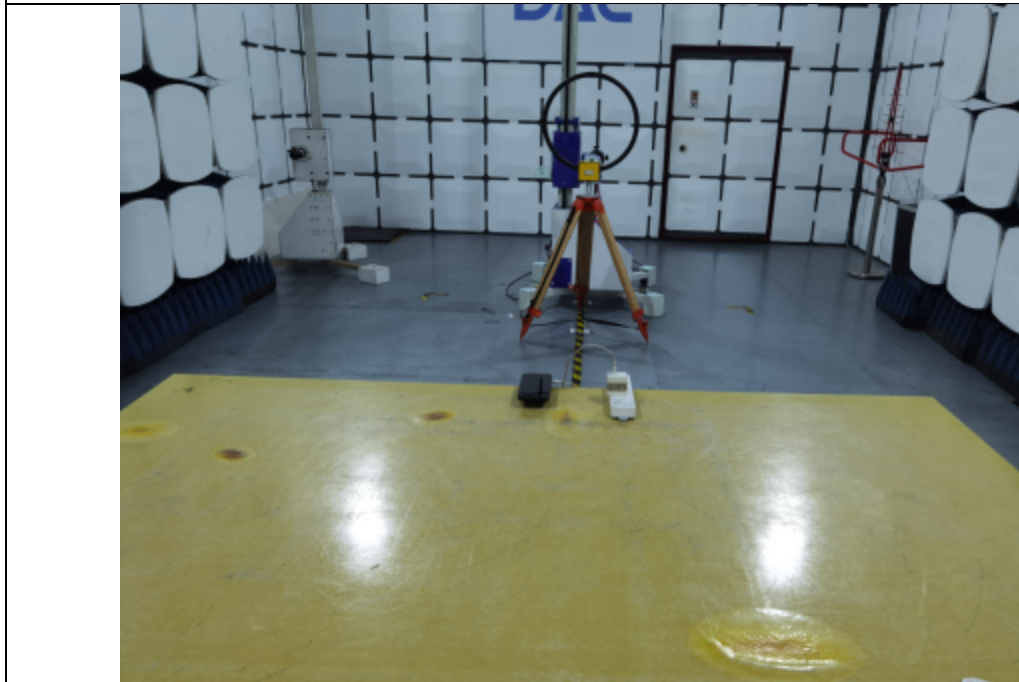
Emissions in frequency bands (below 30MHz) -TM7
