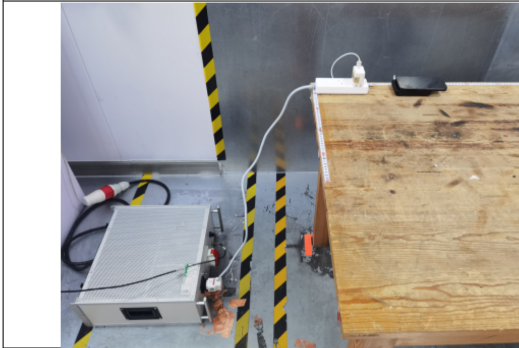
Conducted Emission at AC power line
