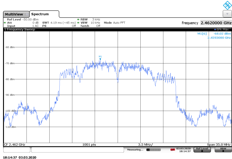
Channel 11 IEEE 802.11n
