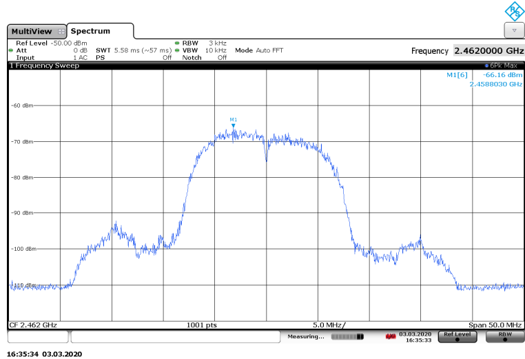
Channel 11 IEEE 802.11g
