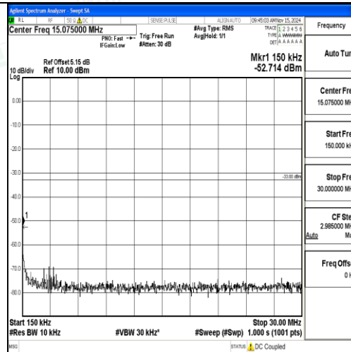
Band2_1.4MHz_16QAM_18607_1RB#0_0.15~30_0.15~30
