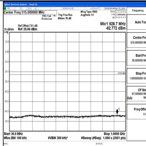
Band2_1.4MHz_16QAM_18607_1RB#0_30~1000_30~1000
