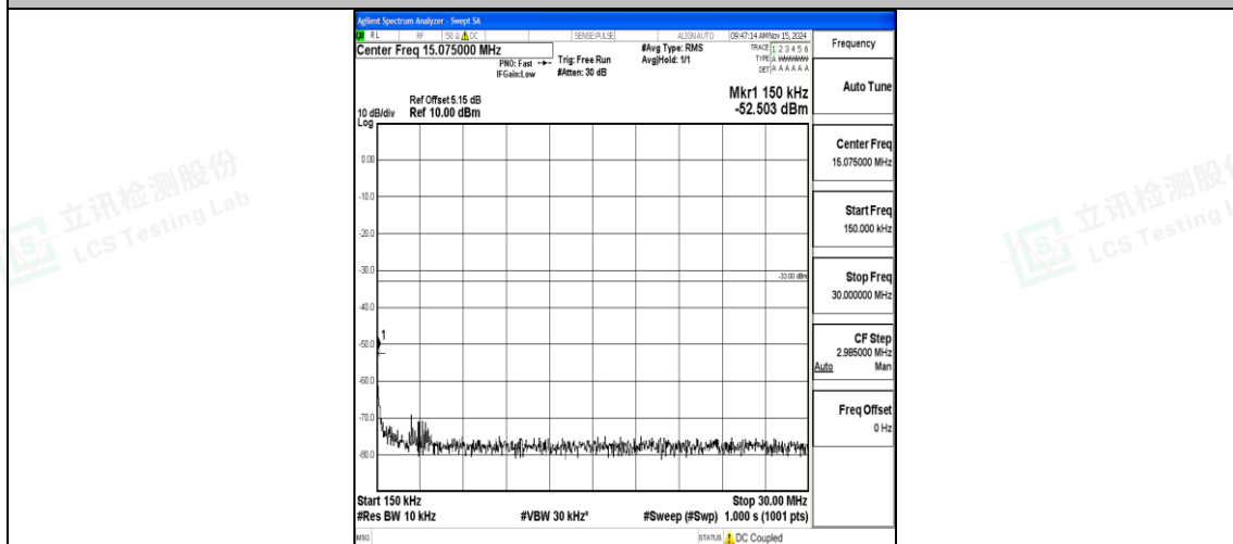
Band2_1.4MHz_16QAM_19193_1RB#0_0.15~30_0.15~30
