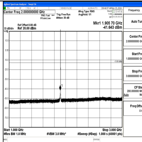
Band2_1.4MHz_QPSK_19193_1RB#0_1000~3000_1000~3000
