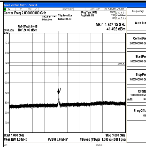
Band2_1.4MHz_16QAM_18607_1RB#0_1000~3000_1000~3000
