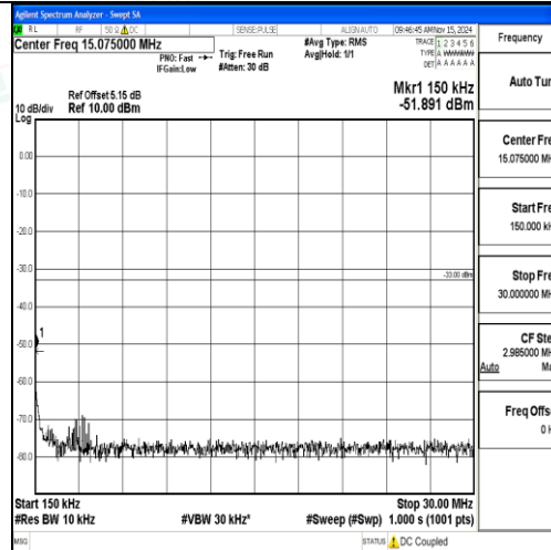
Band2_1.4MHz_QPSK_19193_1RB#0_0.15~30_0.15~30
