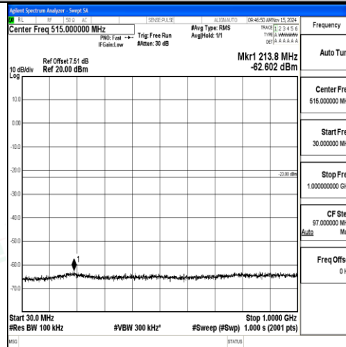
Band2_1.4MHz_QPSK_19193_1RB#0_30~1000_30~1000
