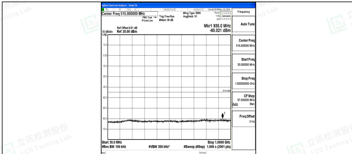
Band7_20MHz_16QAM_21100_1RB#0_30~1000_30~1000
