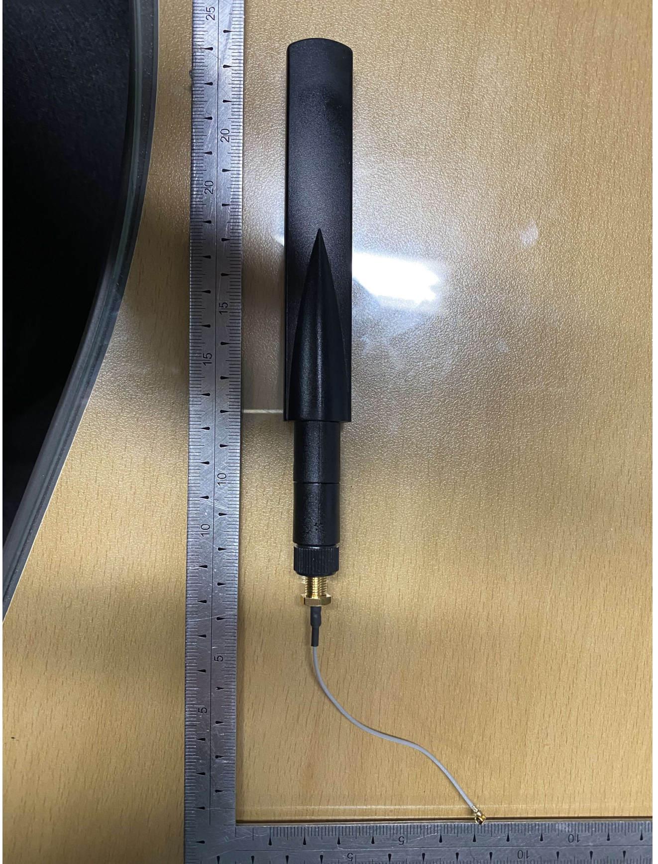
Antenna 1 (Basic) / Dipole Antenna [Model name: AE-T2450/5500DP5-RSMA]
