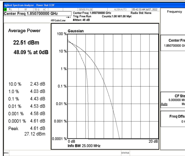
Band2-1.4MHz-QPSK-18607-6RB#0
