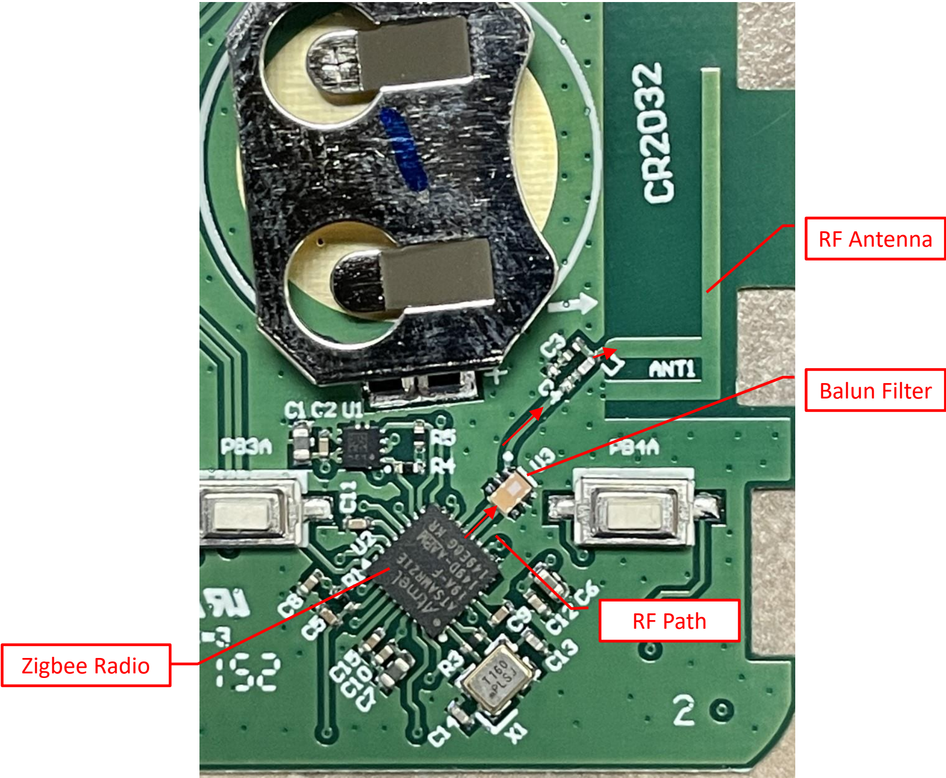
PCBA - RF SECTION
