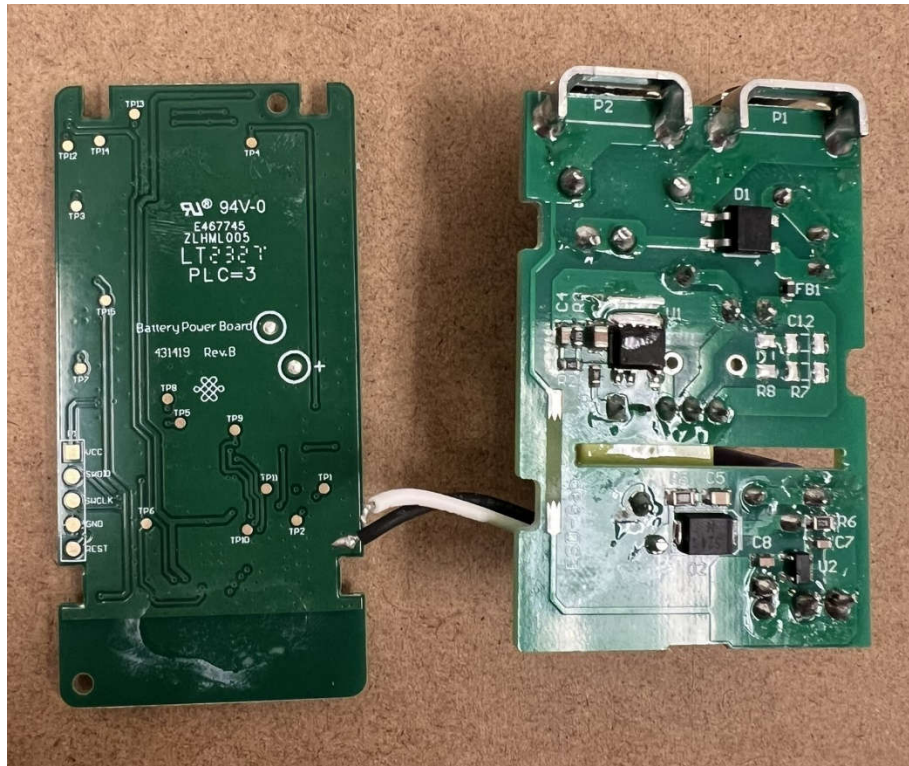
WNRL44 RF Board Back Side (Left) – AC Board Top Side (Right)
