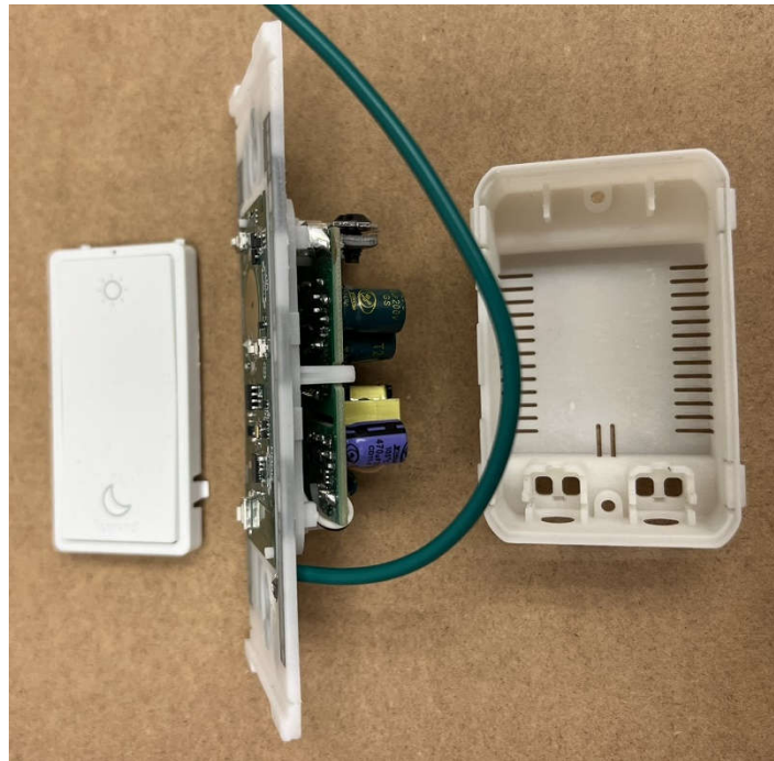
WNRL44 Front and Back Cover Removed
