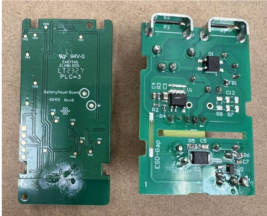
WNRL64 RF Board Back Side (Left) – AC Board Top Side (Right)
