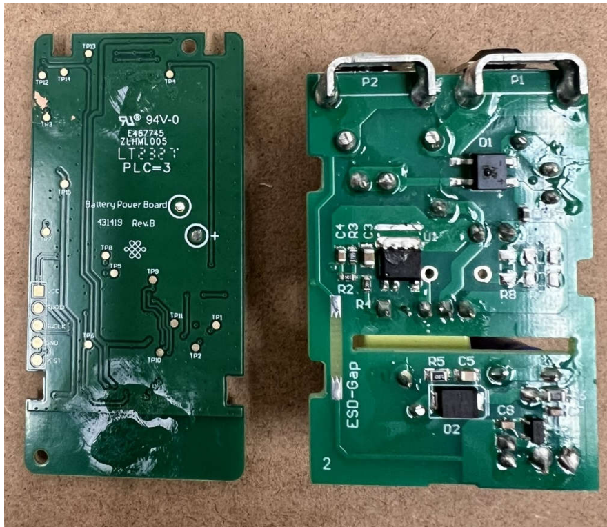
WZ3RL24 RF Board Back Side (Left) – AC Board Top Side (Right)
