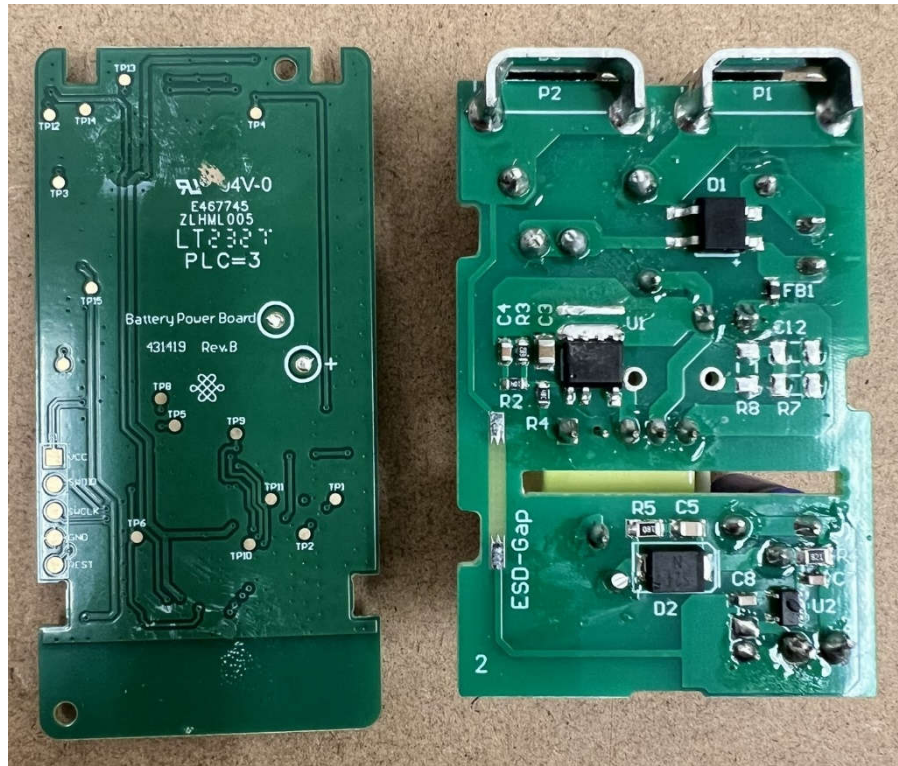
WZ3RL34 RF Board Back Side (Left) – AC Board Top Side (Right)
