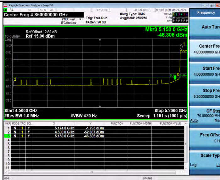
11AC40MIMO_Ant1_Low_5190_Peak
