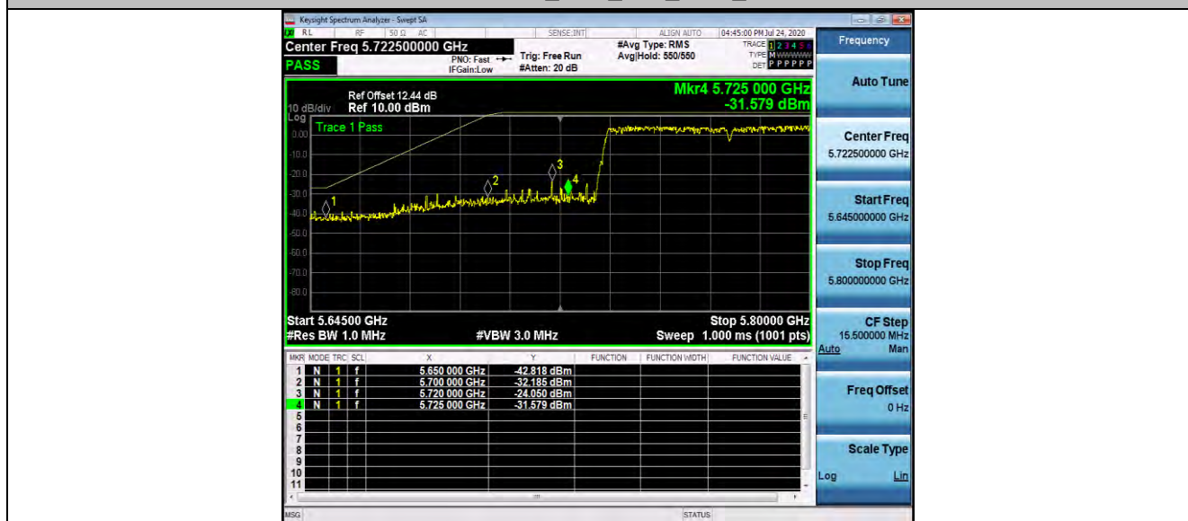
11AC80MIMO_Ant1_High_5775_Peak
