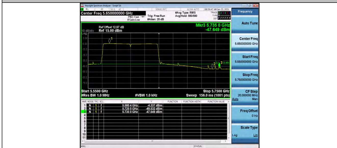
11AC80MIMO_Ant1_High_5610_Peak
