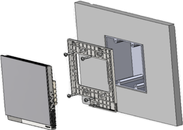
Figure 3 – Flush Mounting
