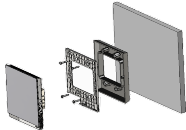
Figure 4 – Wall Mounting
