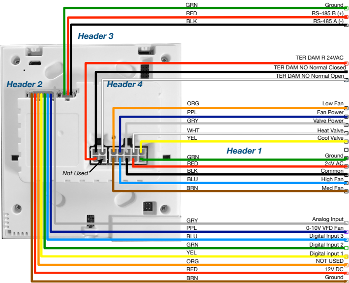
Figure 5 – Wiring Harness Locations
