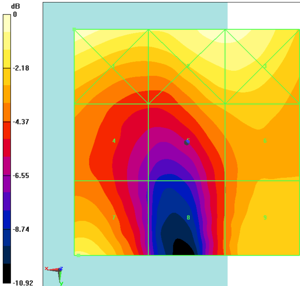
Fig B.15 HAC RF E-Field LTE Band41 16QAM CH40185
