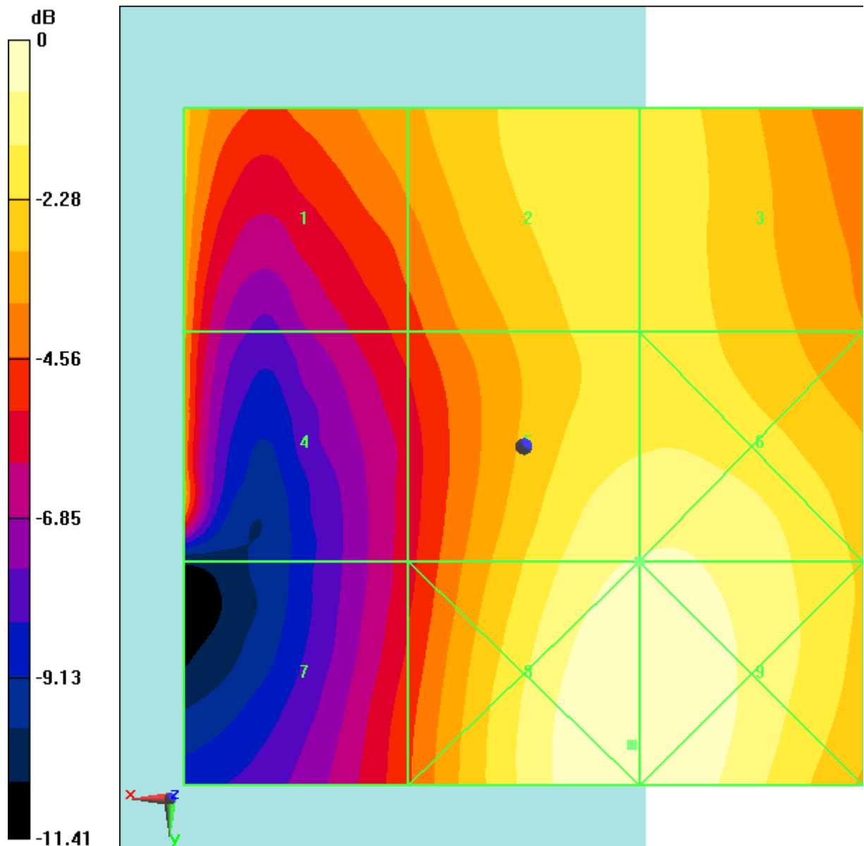
Fig B.5 HAC RF E-Field GSM 1900 Middle
