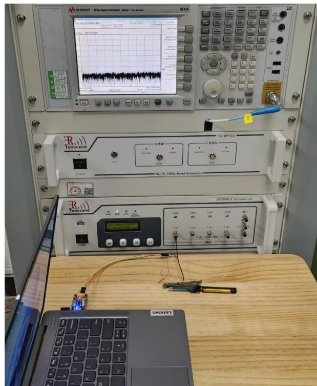
Test Setup Photo(s) of RF Conducted
