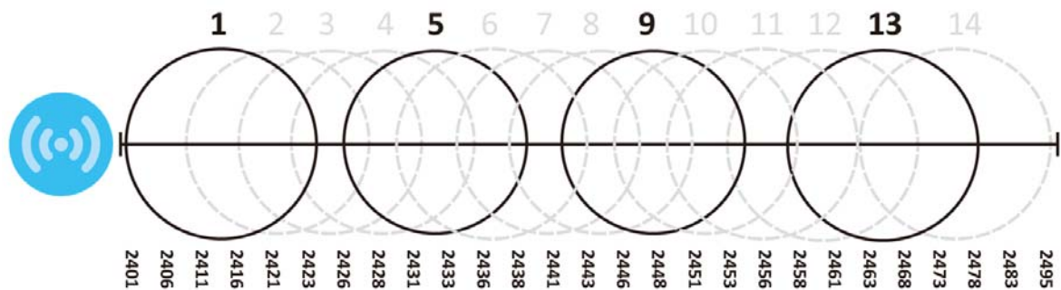
Figure 95 An Alternative Four-Channel Deployment
