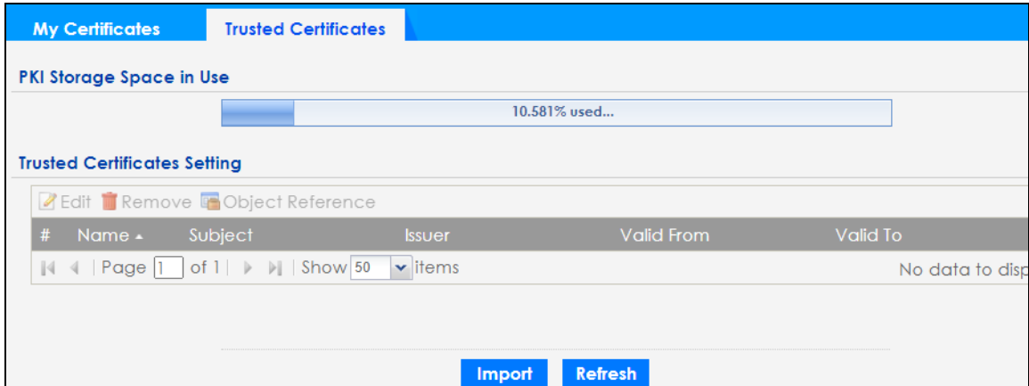
Figure 141 Trusted Certificates
