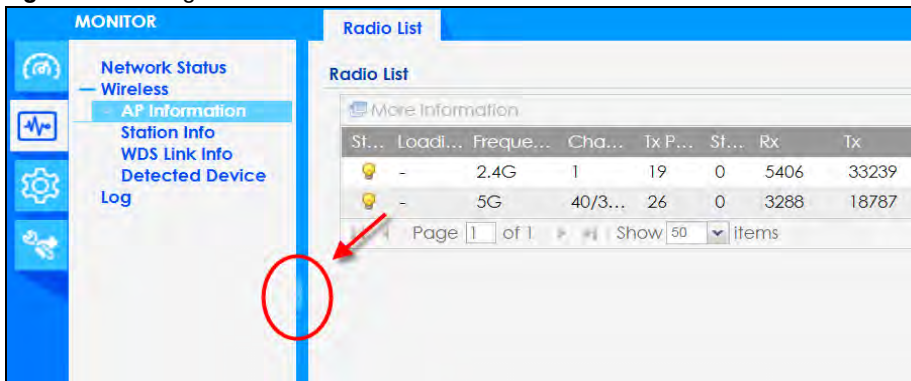
Figure 36 Navigation Panel
