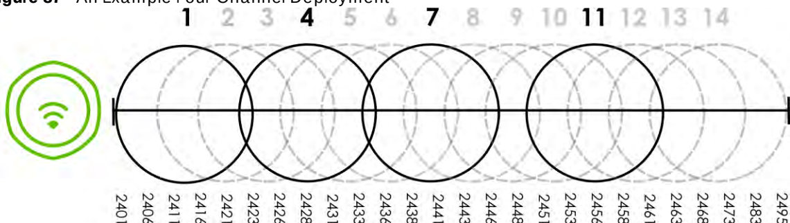
Figure 87 An Example Four-Channel Deployment
