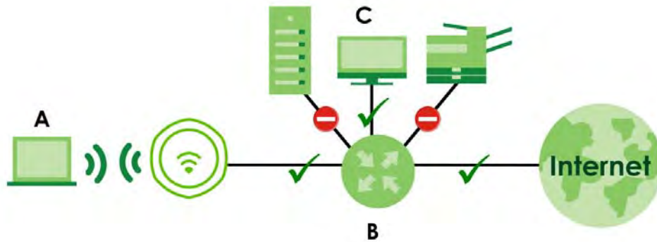
Figure 115 Layer-2 Isolation Application
