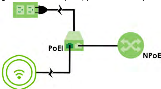
Figure 30 PoE Example Application - PoE Injector
