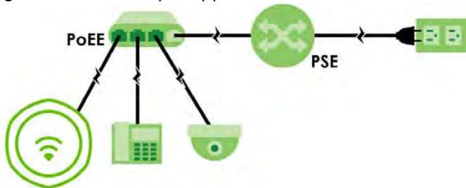
Figure 29 PoE Example Application - PSE with PoE Extender
