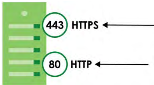
Figure 132 HTTP/HTTPS Implementation
