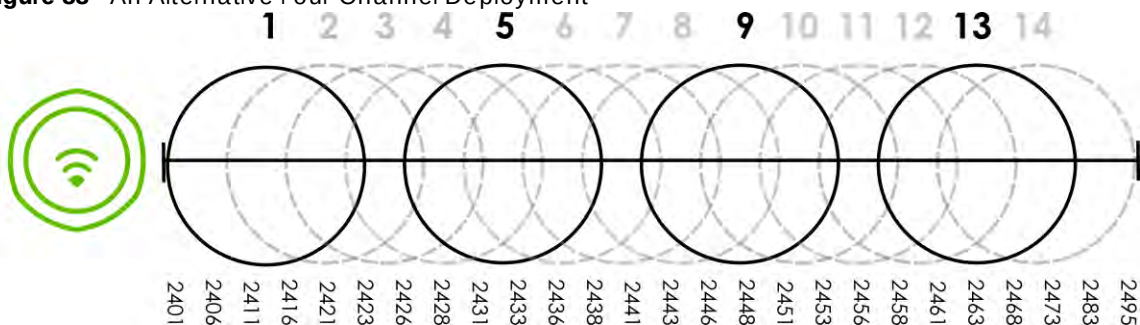
Figure 88 An Alternative Four-Channel Deployment
