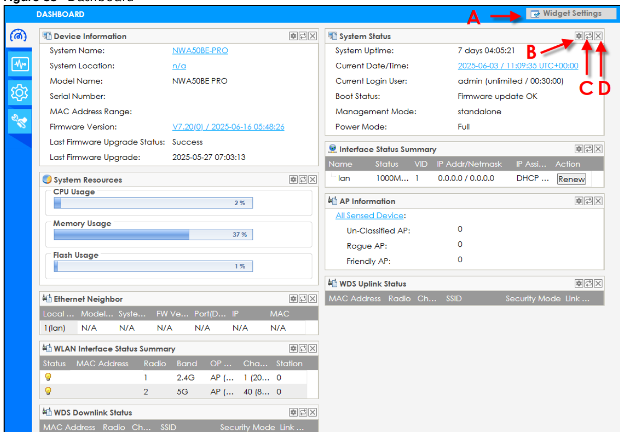
Figure 38 Dashboard
