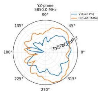
Antenna: 5G-1 Frequency: 5850.0, 5895.0 MHz
