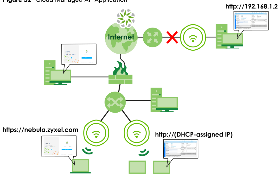
Figure 32 Cloud Managed AP Application
