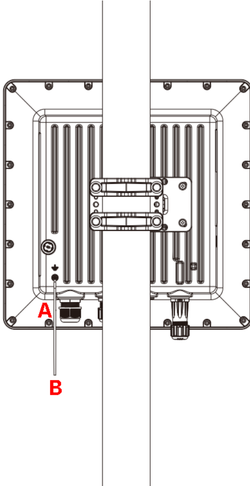
Figure 17 Grounding Example
