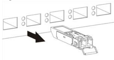
Figure 28 Transceiver Removal Example
