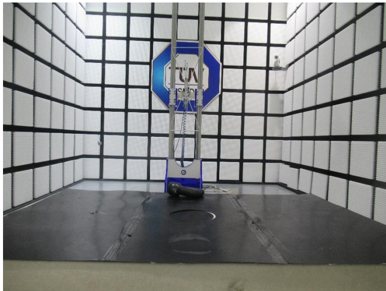
Test Setup – Spurious emissions (30-1000 MHz)
