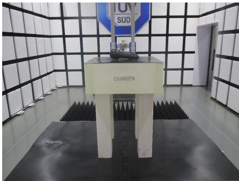
Test Setup – Spurious emissions (Above 18000 MHz)
