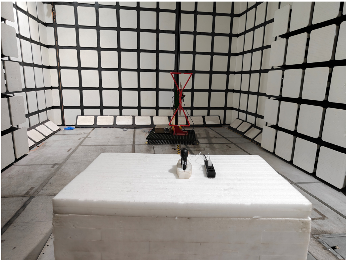
Radiated Emissions View (30 MHz- 1 GHz)
