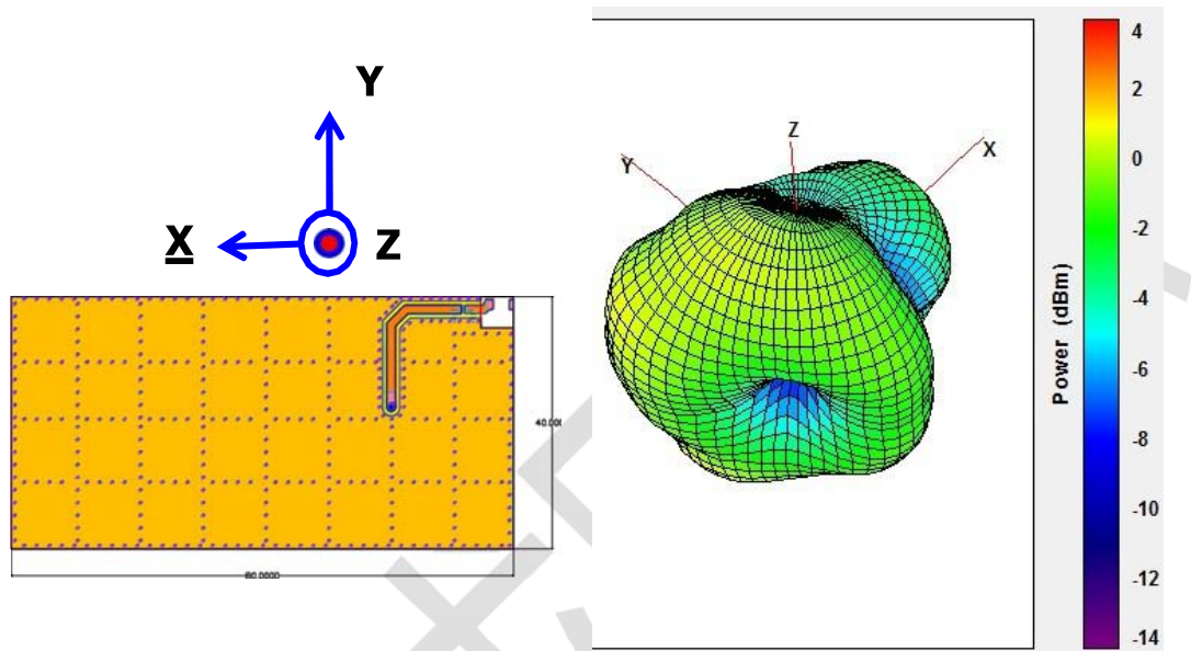
Radiation Pattern
