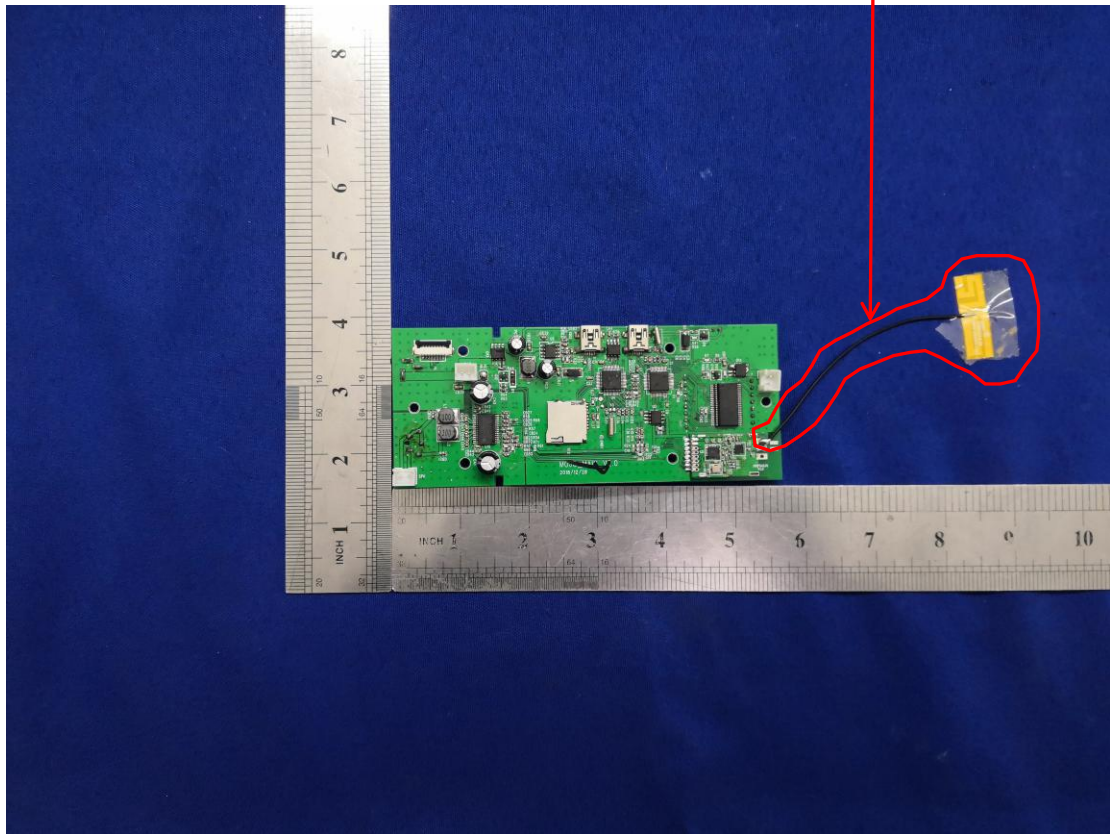
2.4G: FPC Antenna
