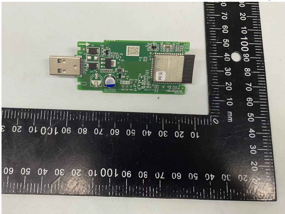
Figure 1 PCB Board (Component Side)
