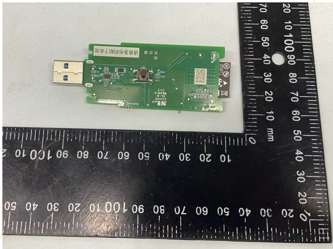
Figure 2 PCB Board (Solder Side)
