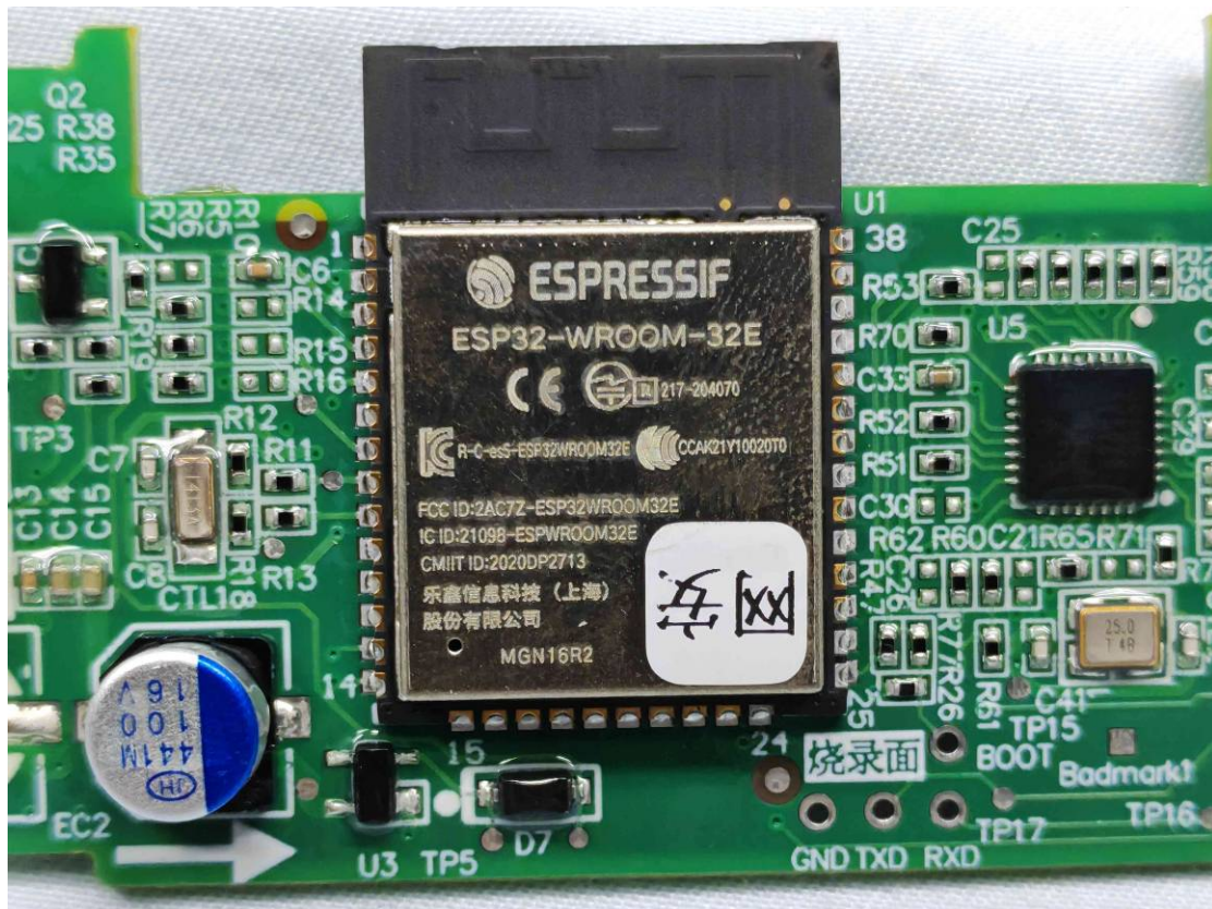
Figure 3 Wireless Module
