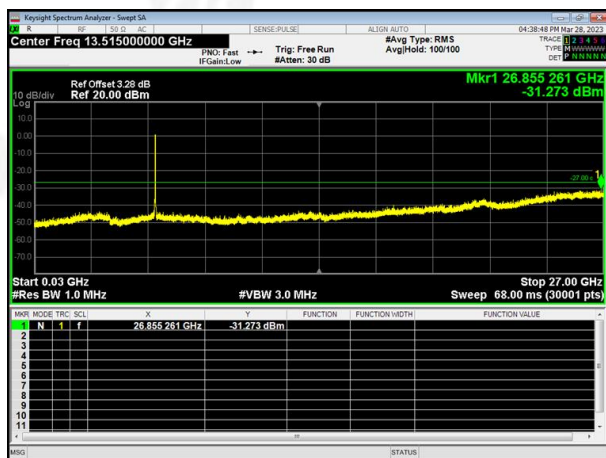
802.11n20 on channel 151
