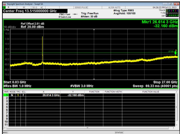
802.11n on channel 48
