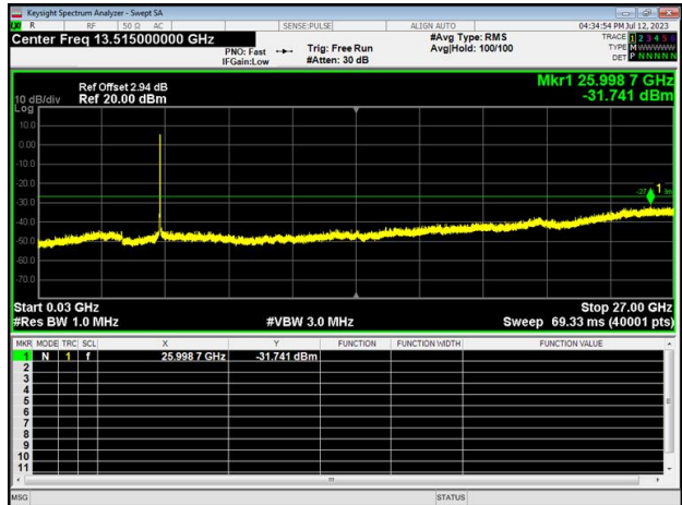
802.11n on channel 48
