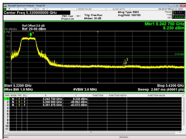
(802.11a) Band Edge, Right Side
