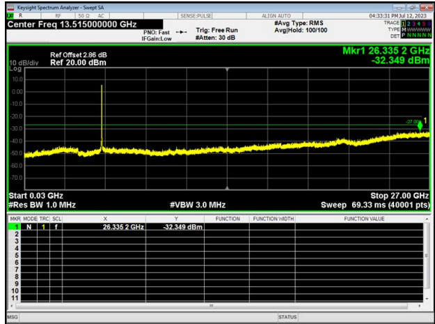
802.11n on channel 40
