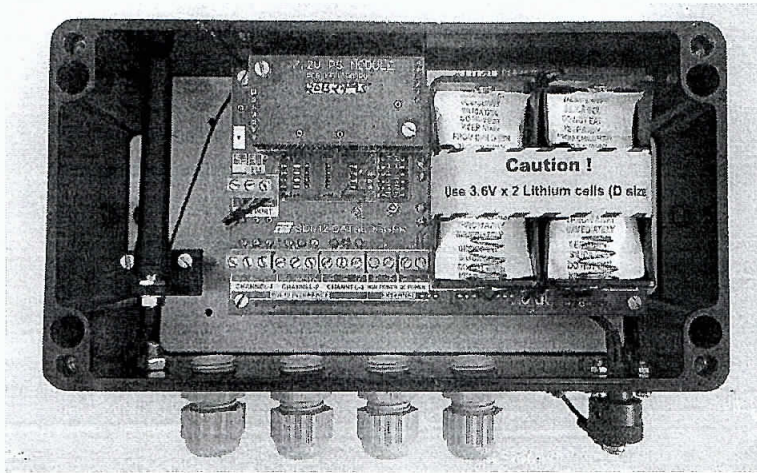
Model: ESDL-30-3V0-4GUS
