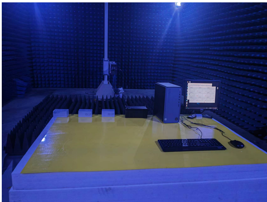
(Above 1G) Front View
