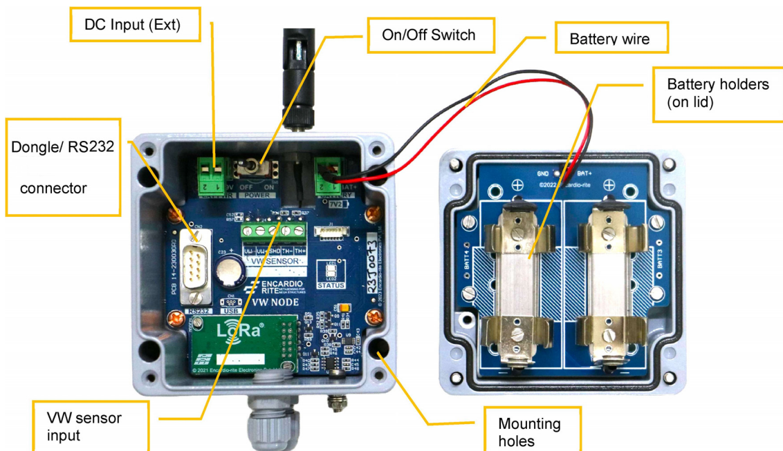
Figure 5-2 Node details
