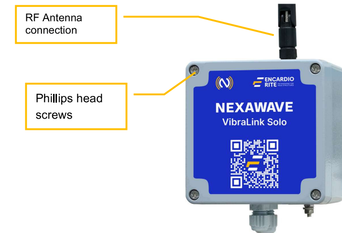
Figure 5-1 VW node
