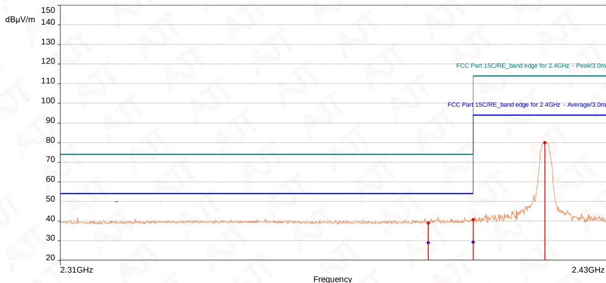
2416MHz Vertical
