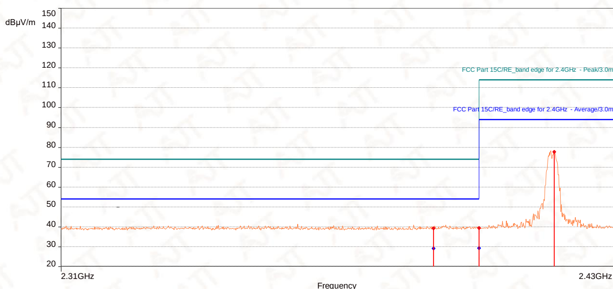
2416MHz Horizontal
