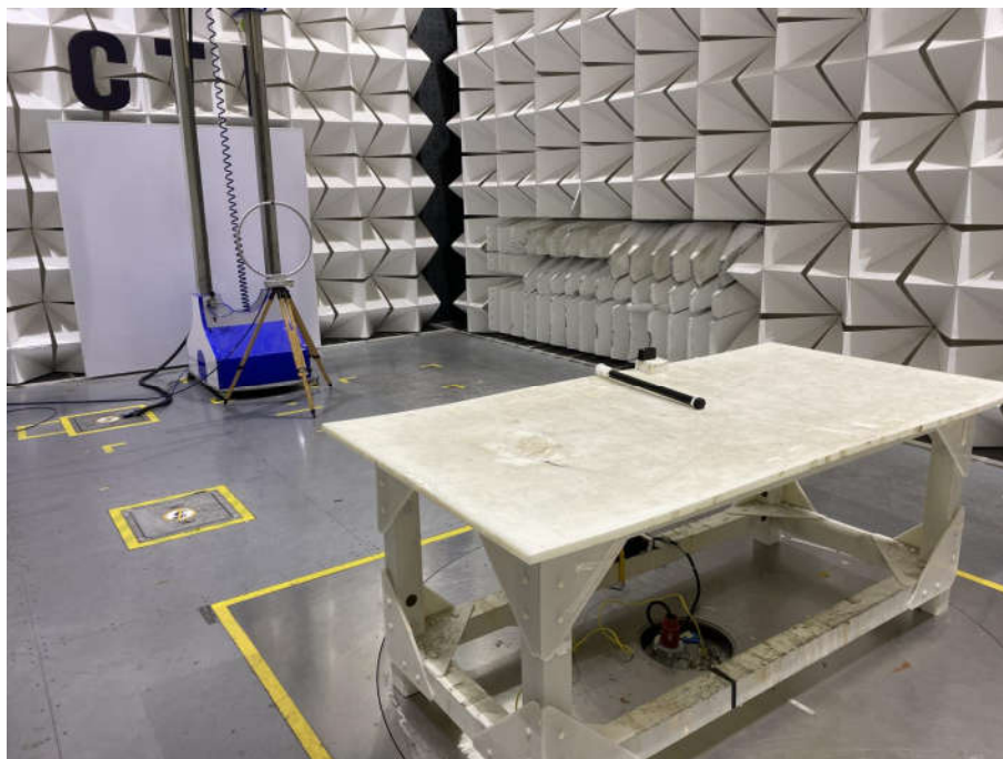
Radiated emission Test Setup-1(Below 30M)
