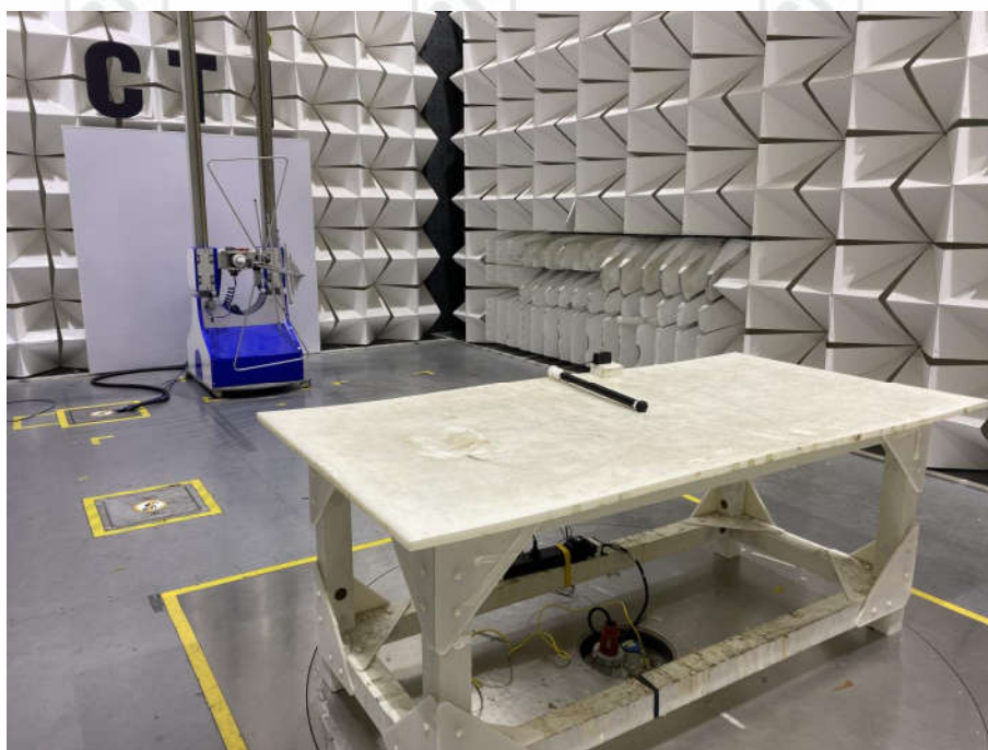
Radiated emission Test Setup-2 (Below 1G)
