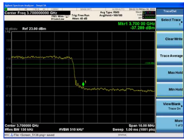
LTE Band 48 64QAM 20MHz CH-High 1RB
