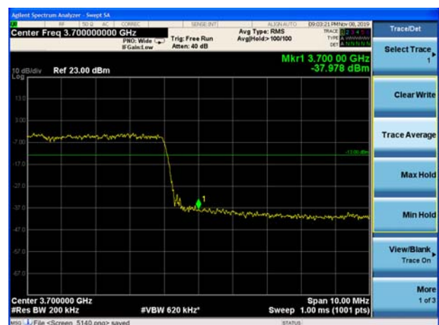
LTE Band 48 64QAM 20MHz CH-High 100%RB
